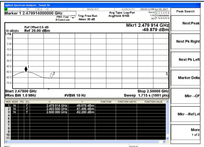
BT LE-High channel(AV)
