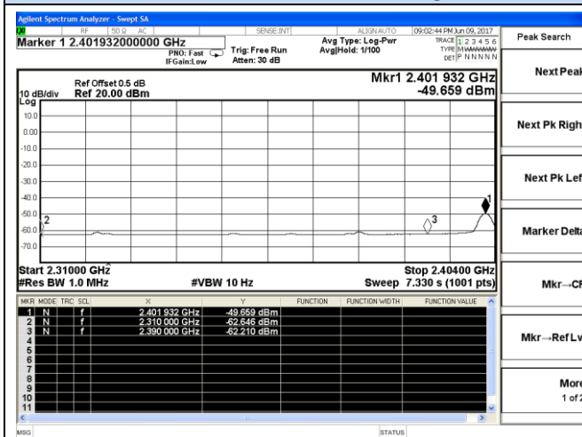
BT LE-Low channel(AV)
