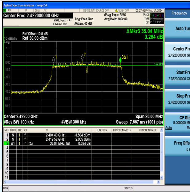
11N40MIMO-Ant2-2422-PASS
