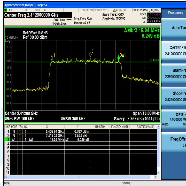
11AX20MIMO-Ant2-2412-PASS
