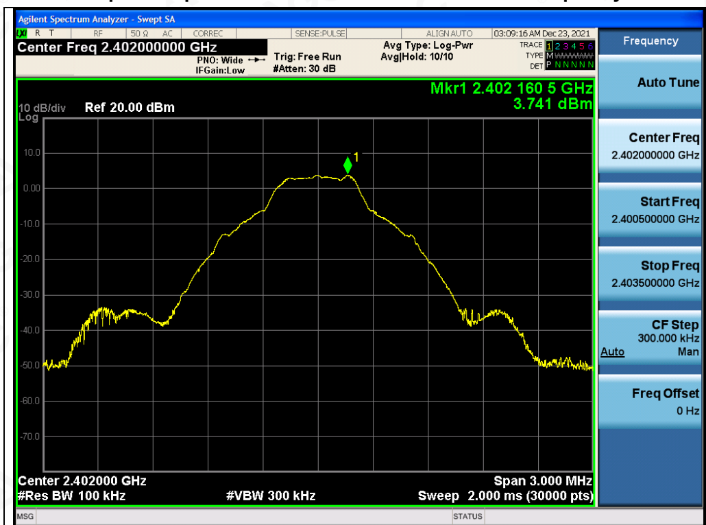
Test Graph BR ANT1 2402 1Mbps Reference Level
