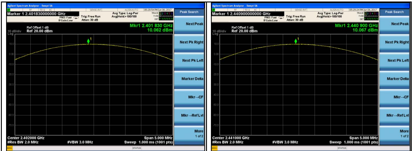
8DPSK Output power - Low CH 2402
