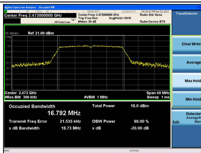
802.11g 20dB Bandwidth - CH 13
