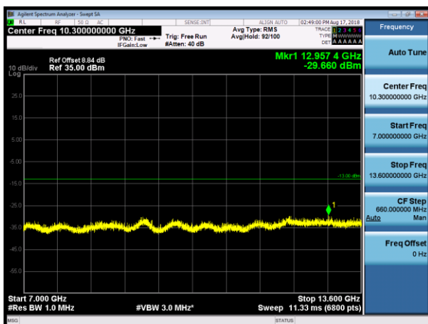
GSM 1900-MCH-GSM
