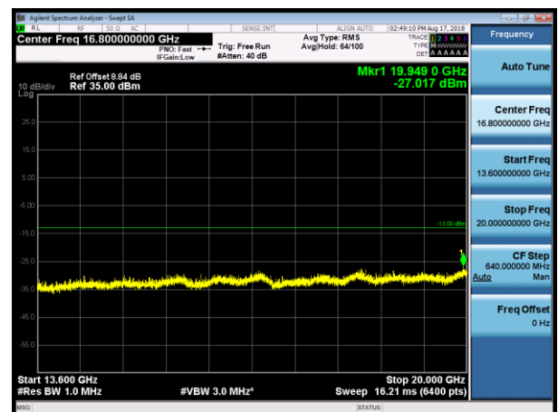
GSM 1900-MCH-GSM
