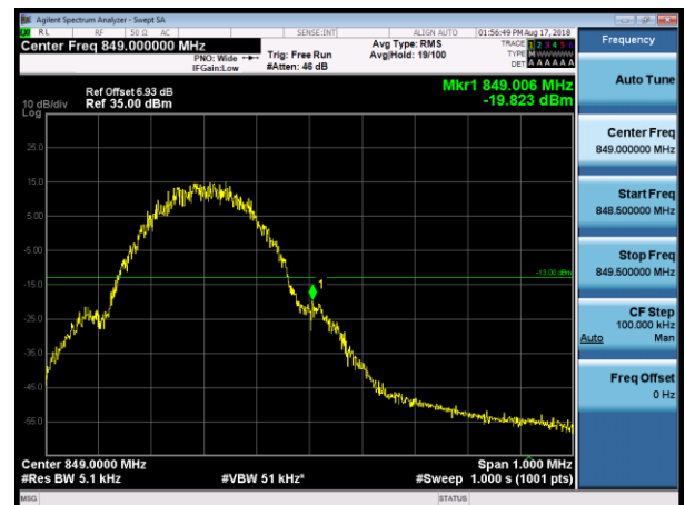
GSM 850-HCH-EDGE
