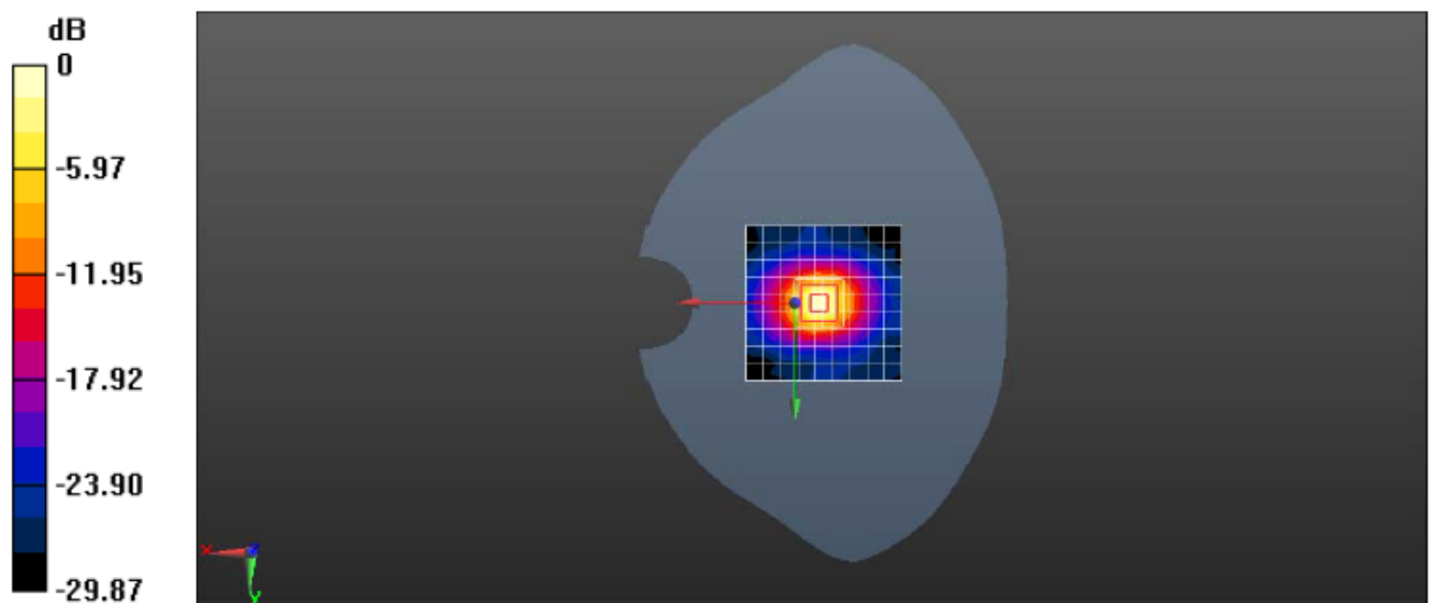
System Performance Check 5600 MHz 100mW
