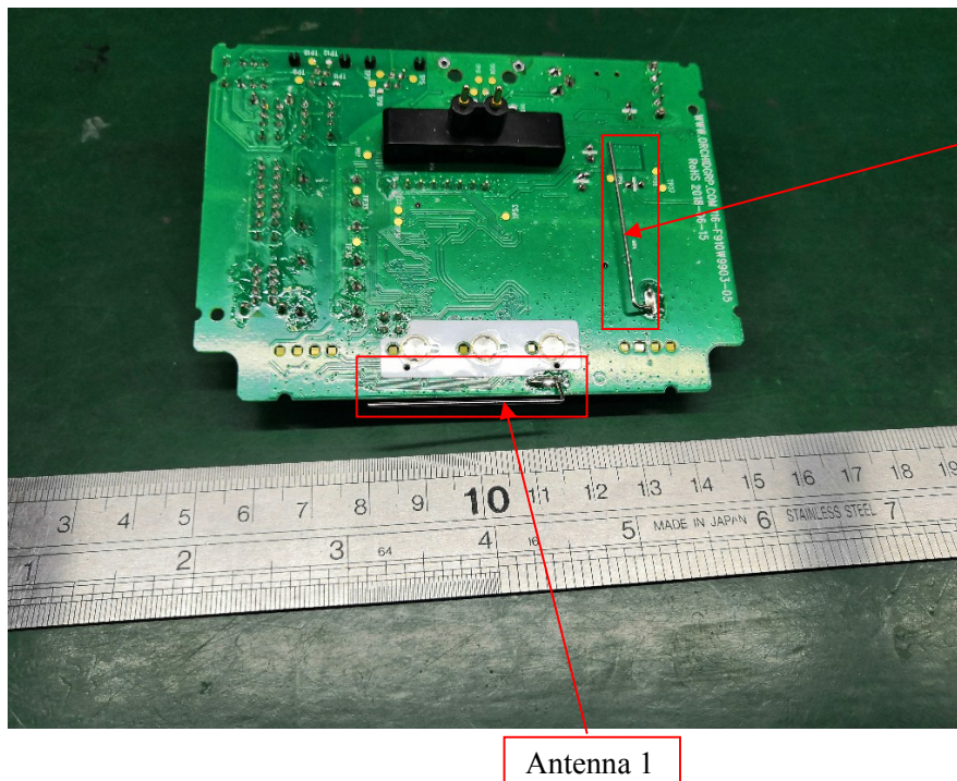
EUT – Main Board Bottom View
