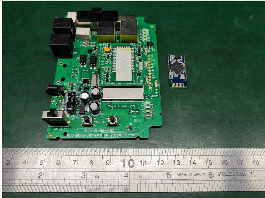
EUT – Main Board Top View 3 (Bluetooth Module Unloaded)
