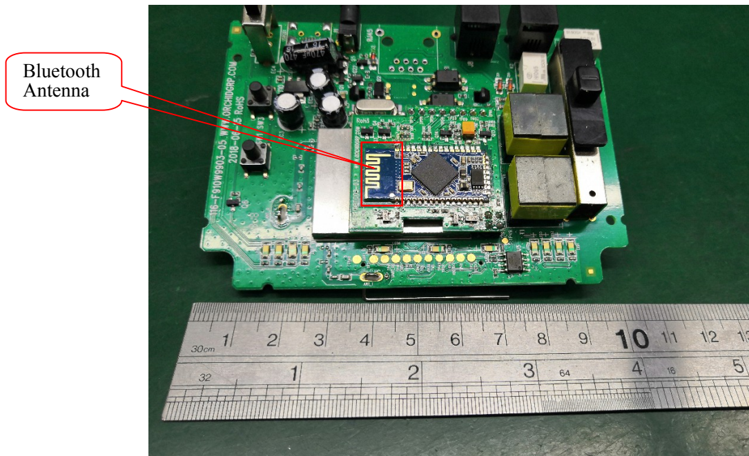
EUT – Main Board Top View 2 (Shielding off)
