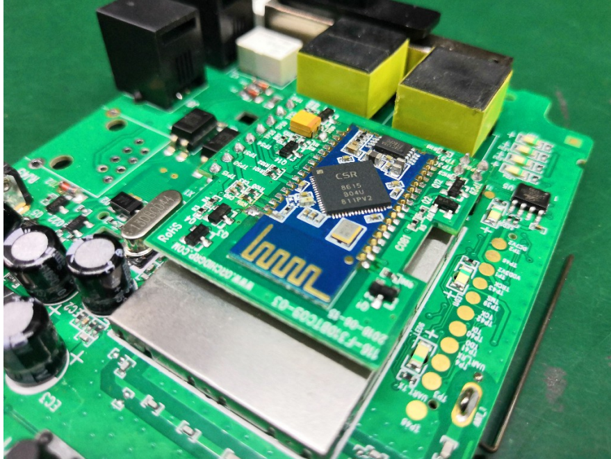
EUT – Main Chip View (for Bluetooth Module)
