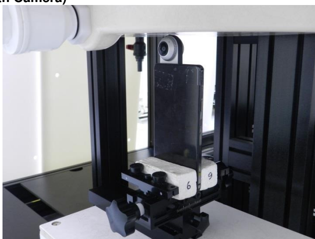
Top side with 0 mm separation distance (Phone with Camera)
