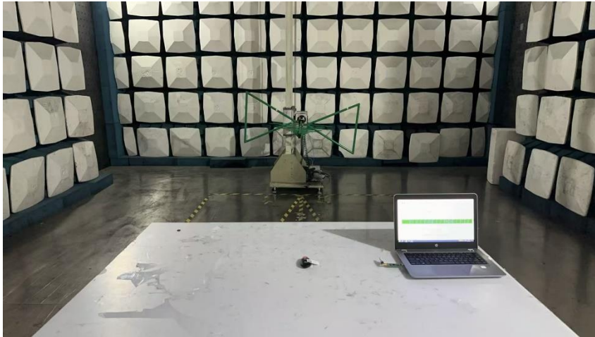
Radiated Emissions below 1GHz
