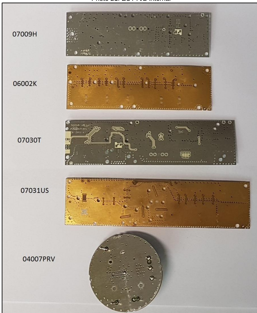
Photo 21: EUT A/B internal
