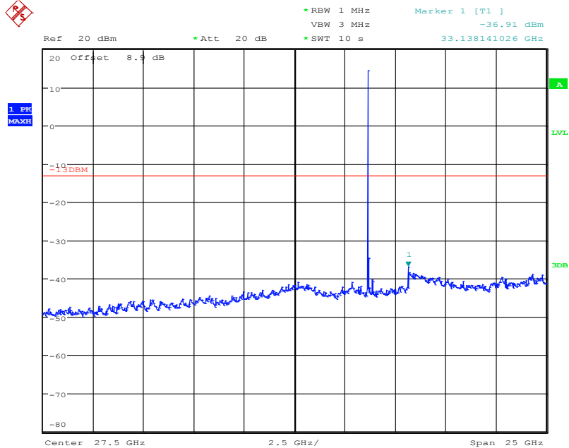
Plot No. A.25: QPSK, conducted spurs
