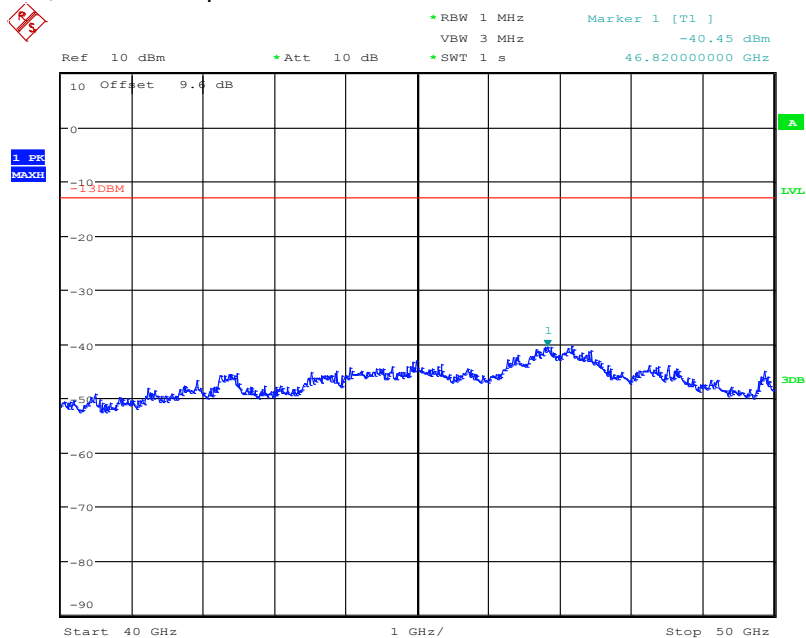
Plot No. B.26: QPSK, conducted spurs
