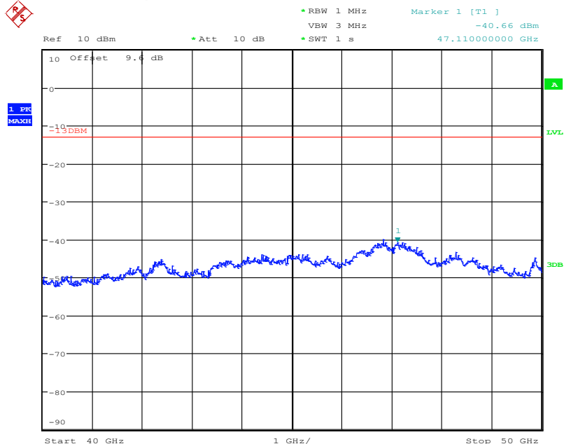
Plot No. A.26: QPSK, conducted spurs
