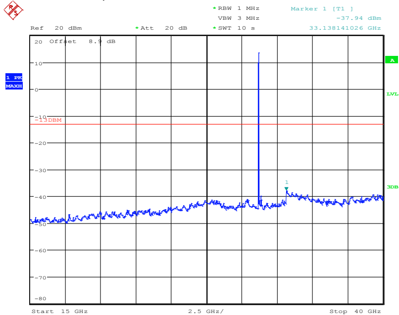
Plot No. B.25: QPSK, conducted spurs
