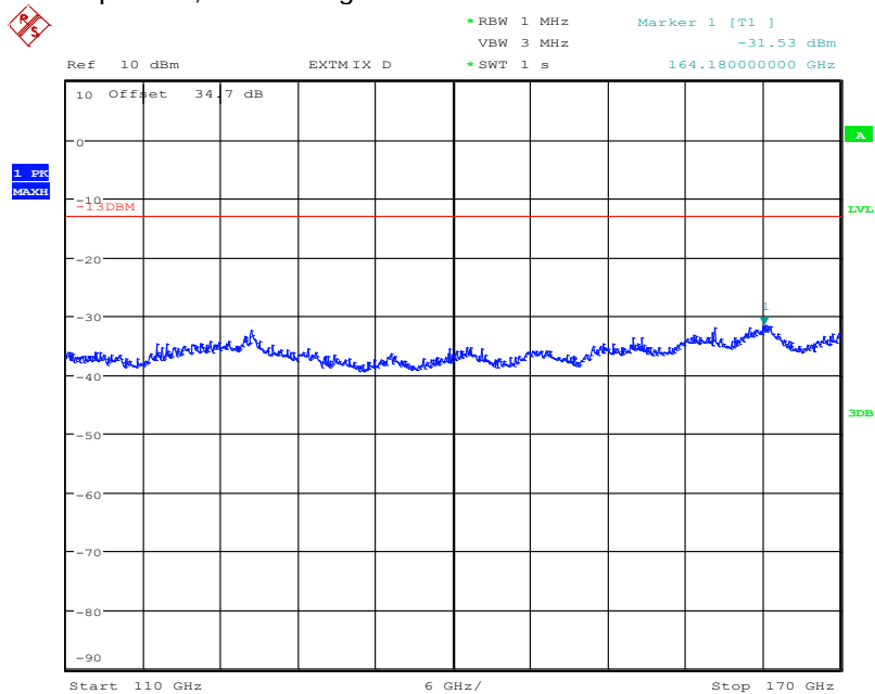
Plot No. B.43: radiated spurious, low/mid/high
