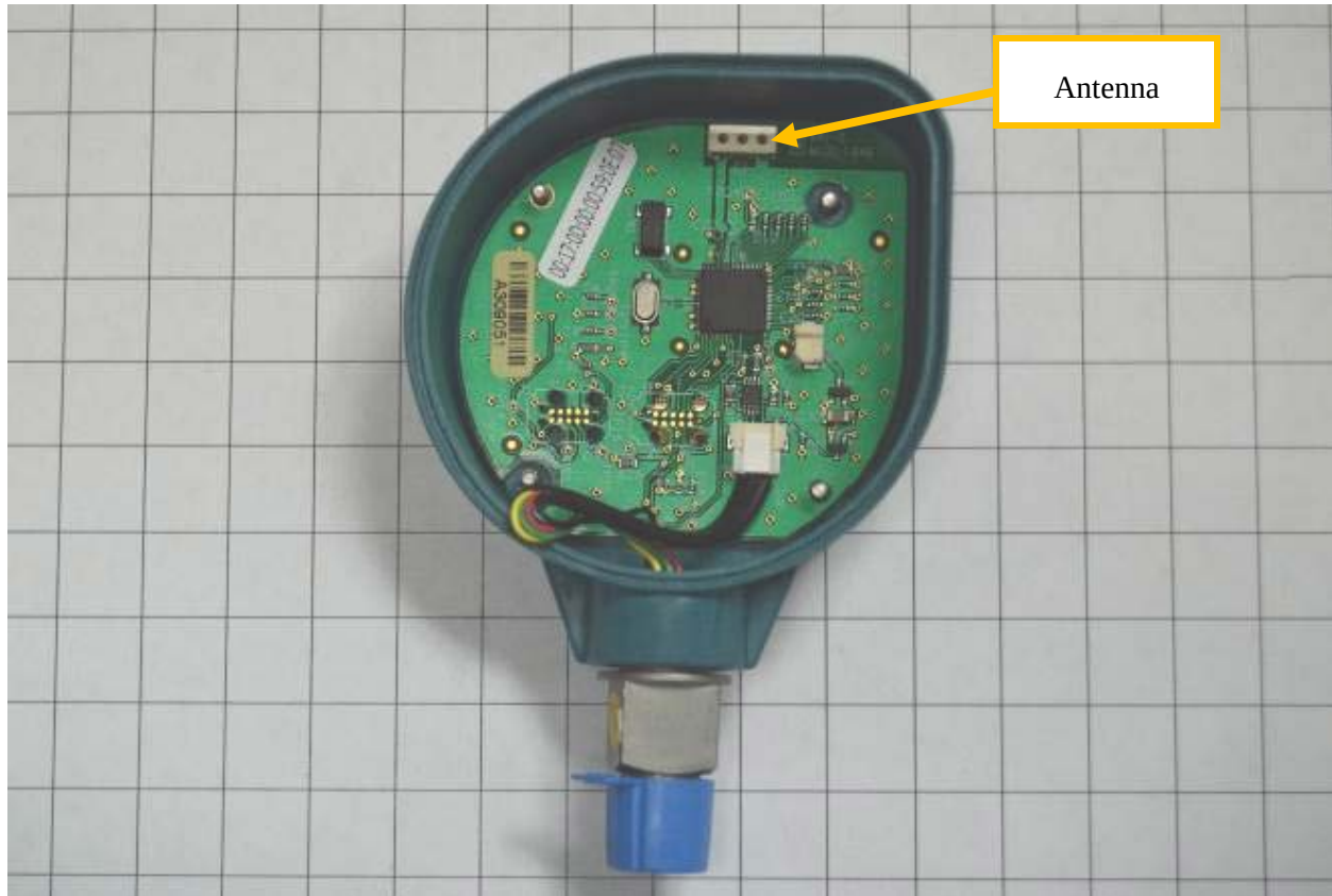
Figure 4: Internal View of Base Housing with Main PCB (Battery Compartment removed) (Photo provided by Airgas)
