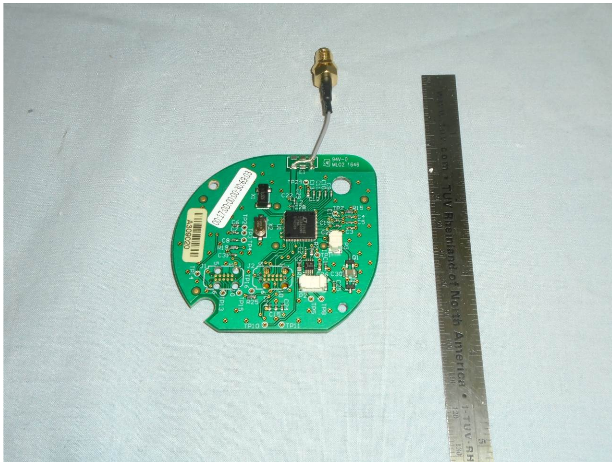
Figure 3: View of Modified EUT with an SMA Connector to allow direct measurement of the transmitter.
