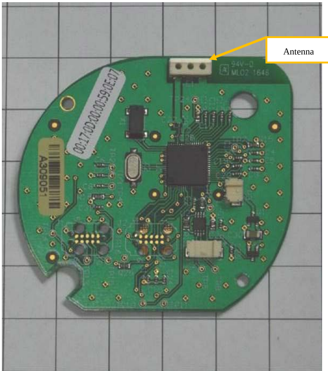
Figure 6: Front View of Circuit Board (Photo provided by Airgas)
