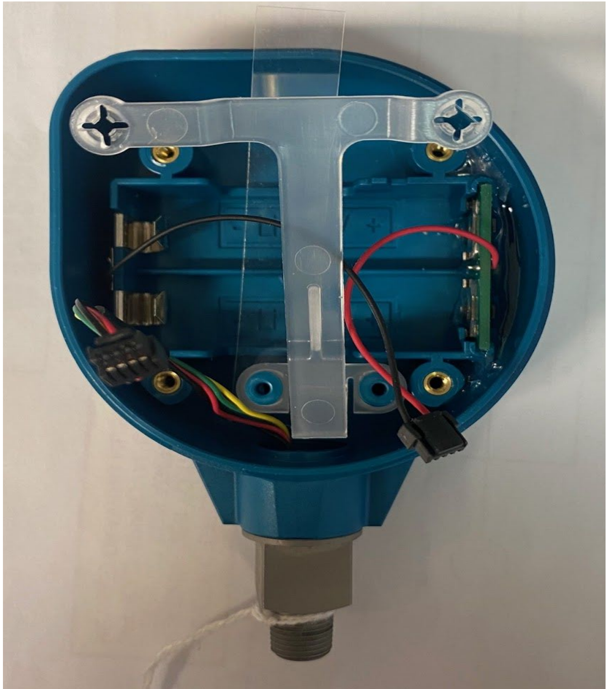
Internal Photos of CAM Pressure Remote Gen 2 Top Open View
