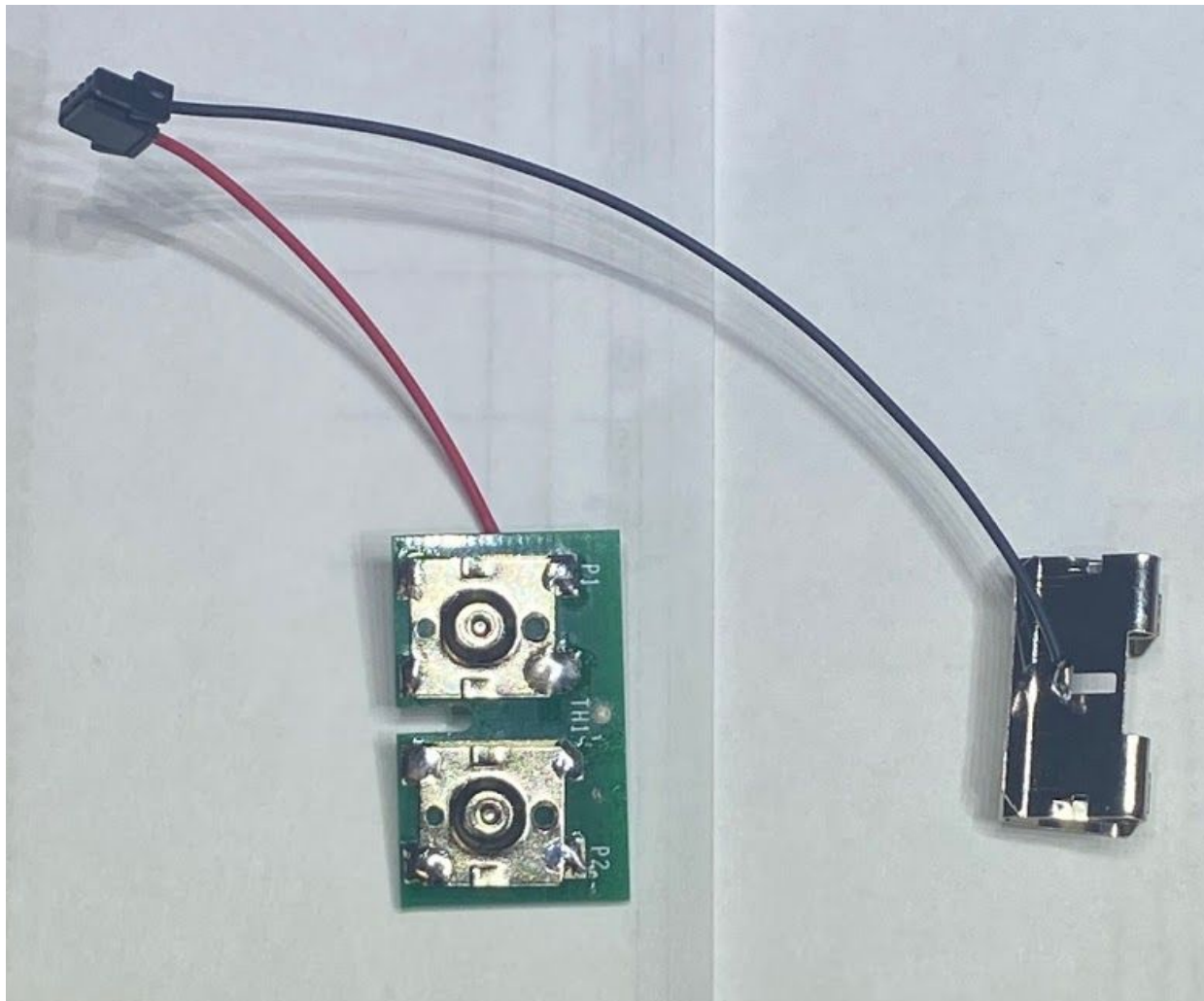
Battery Board Front View
