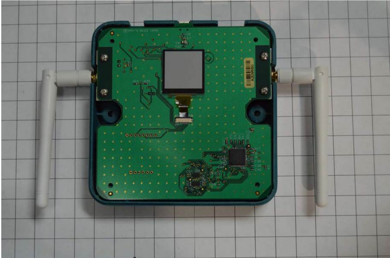
Figure 1: Internal Front View of EUT (Photo provided by Airgas)
