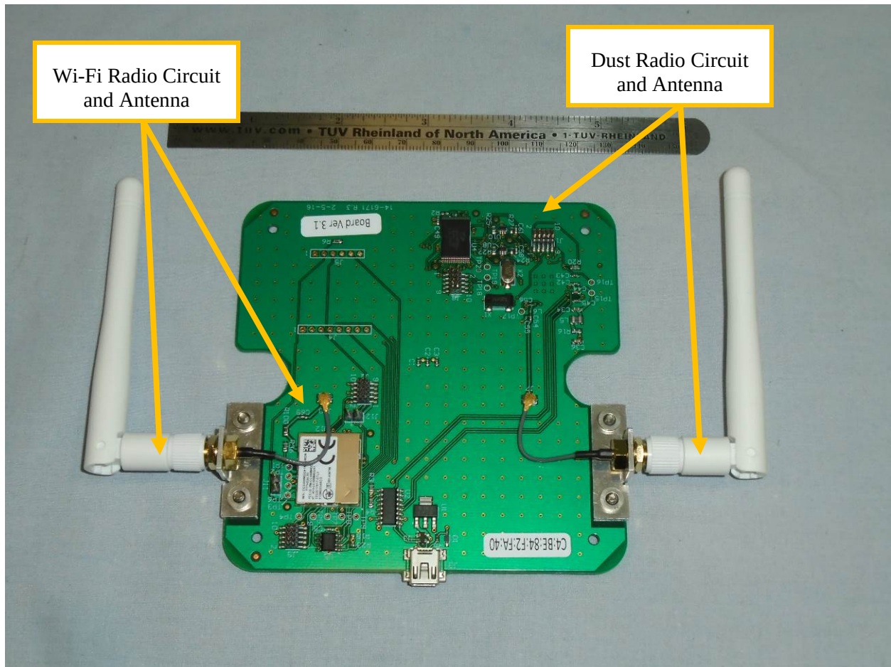
Figure 2: Top Internal Rear View
