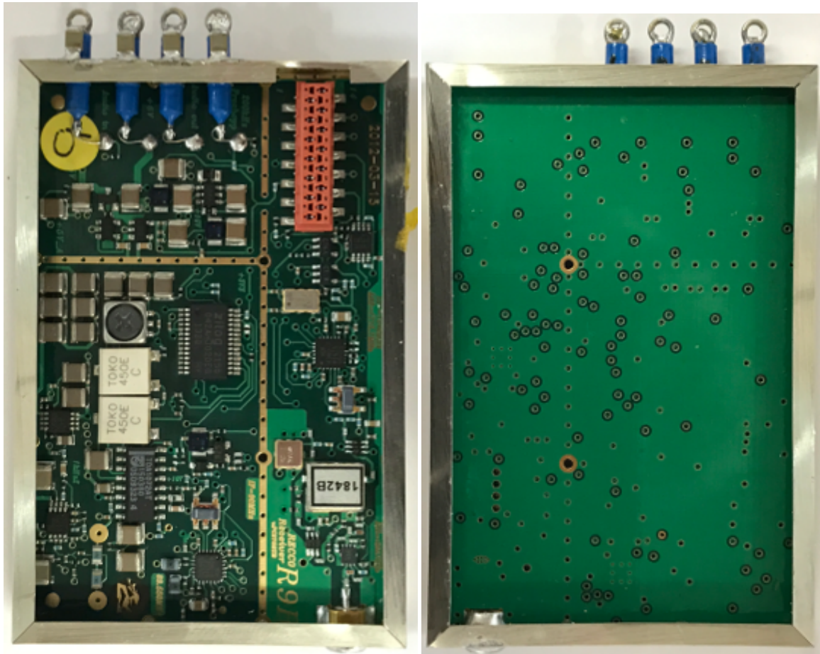
Figure 5: Recco Detector Rx PCB Top and Bottom sides.
