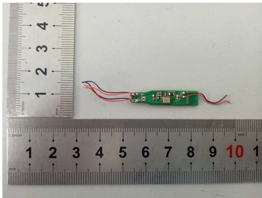
EUT – Earbud-1 PCB Bottom View
