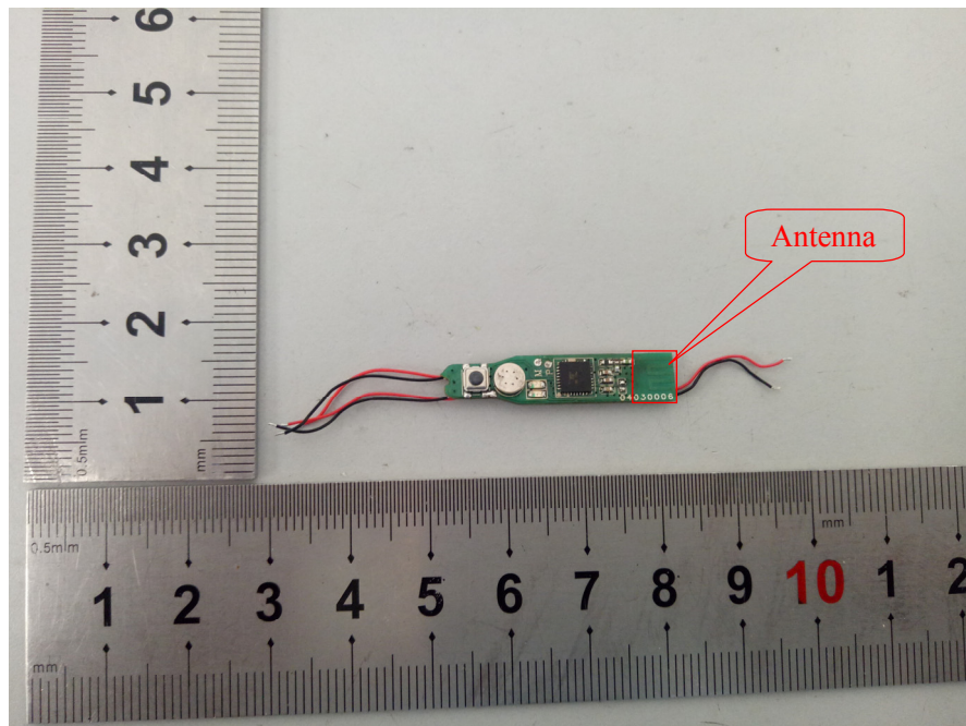
EUT – Earbud-2 PCB Bottom View
