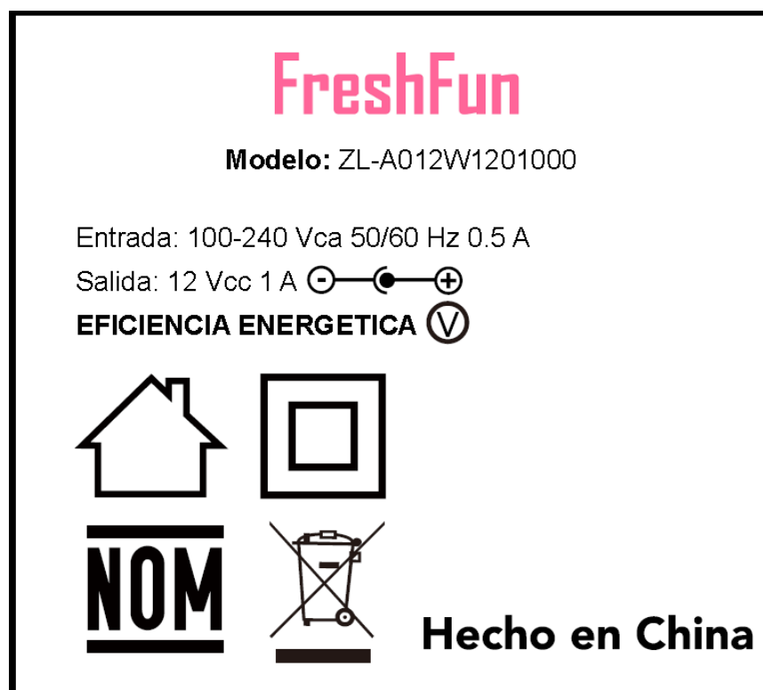
EUT –Adapter Label View
