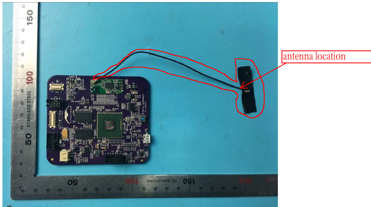
INTERNAL PHOTO OF SAMPLE – 11
