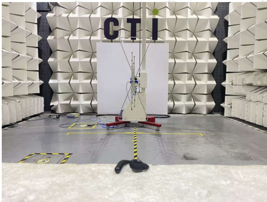
Radiated spurious emission Test Setup-5 Right ear(Below 1GHz) close up
