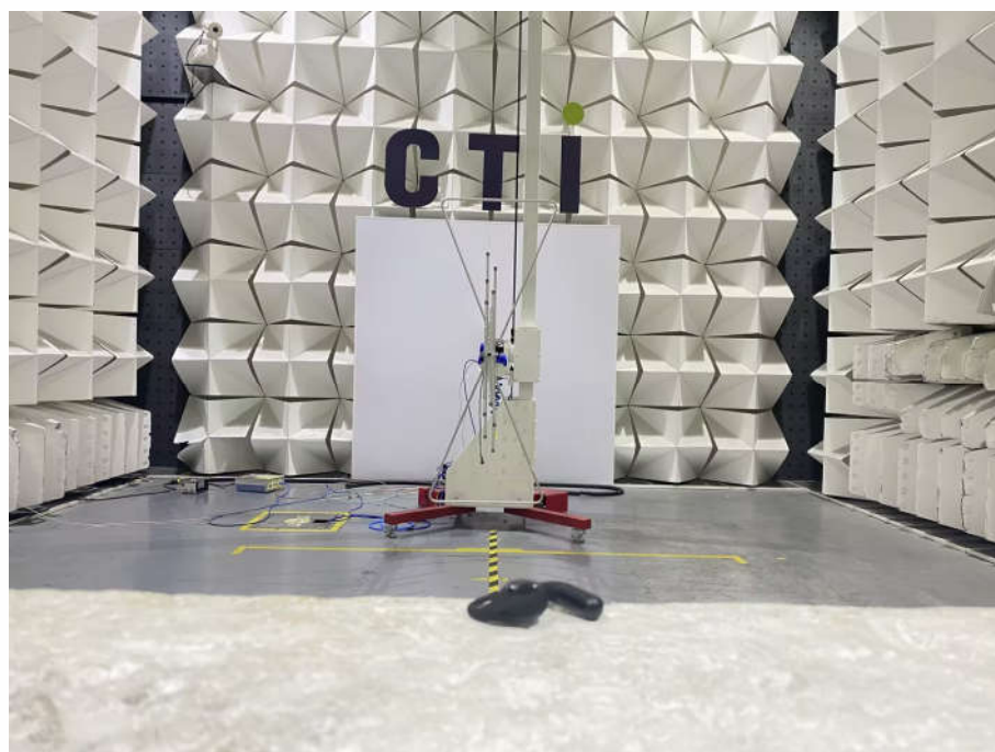
Radiated spurious emission Test Setup-2 Left ear (Below 1GHz) close up
