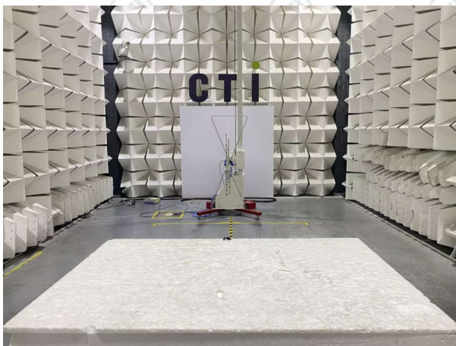
Radiated spurious emission Test Setup-4 Right ear(Below 1GHz)
