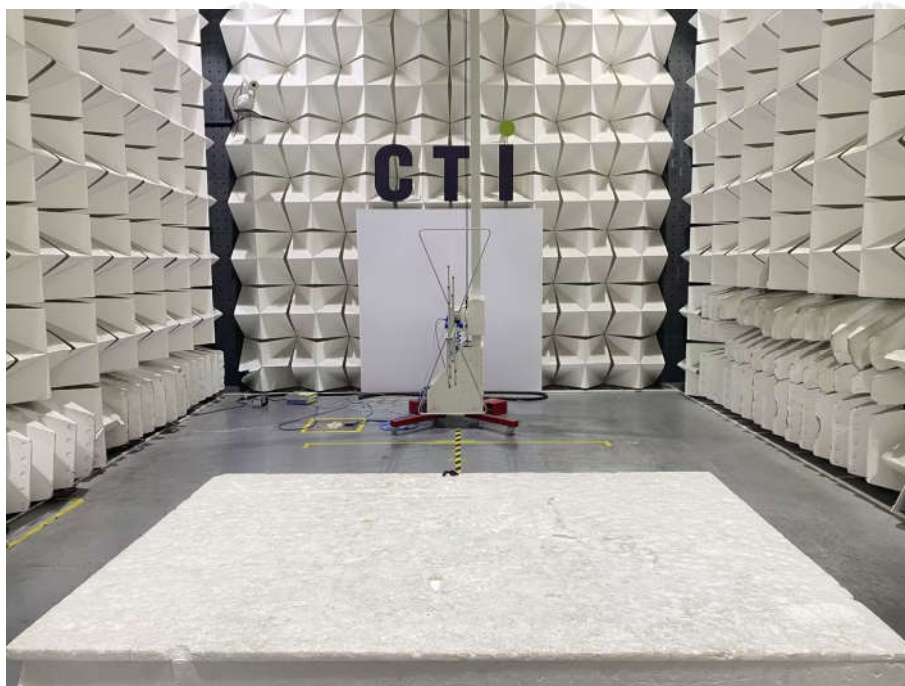
Radiated spurious emission Test Setup-4 Right ear(Below 1GHz)
