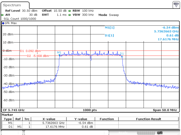
802.11ac20_5745MHz_Chain 1
