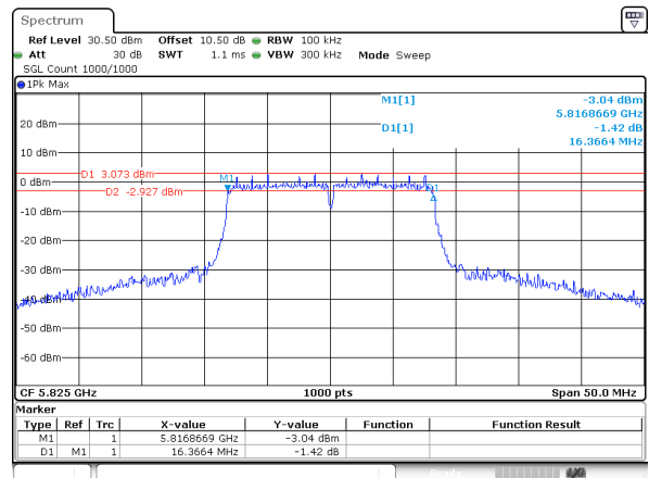
802.11a_5825MHz_Chain 0
