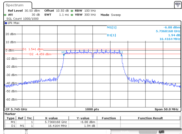
802.11a_5745MHz_Chain 0
