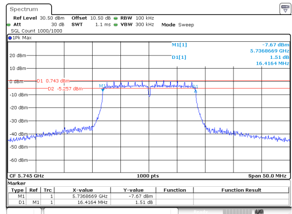
802.11a_5745MHz_Chain 1
