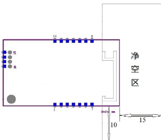
PCBAntenna minimum clearance area
