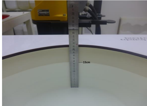
Photo 1: Tissue Simulant Liquid for Head 2450
