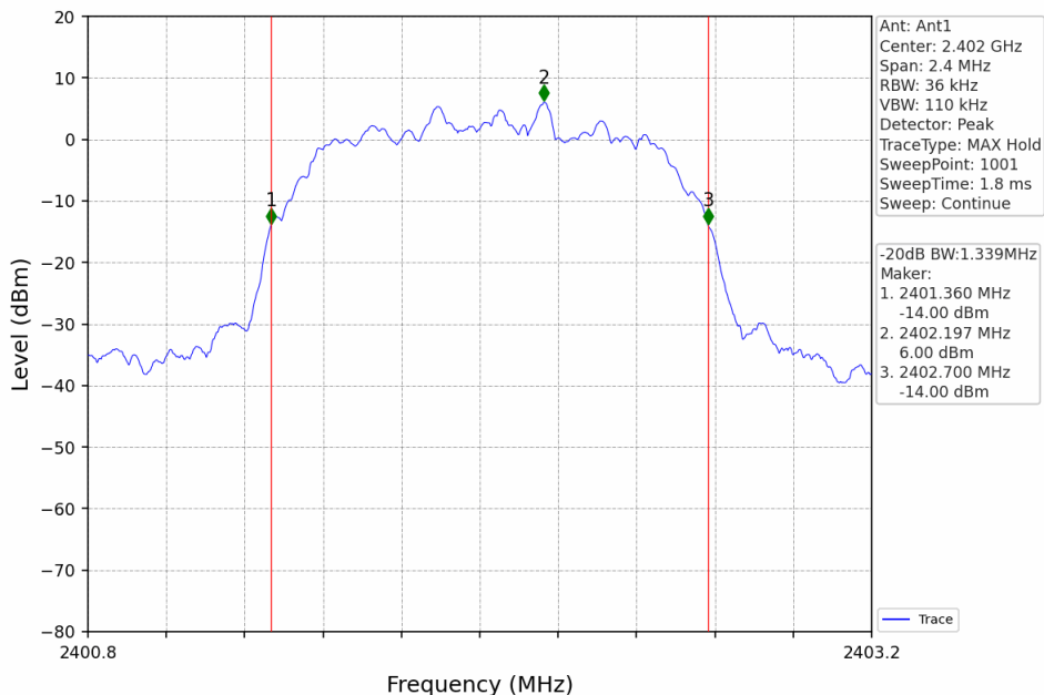
Pi/4DQPSK_2DH5_LCH_2402MHz_Ant1_NTNV
