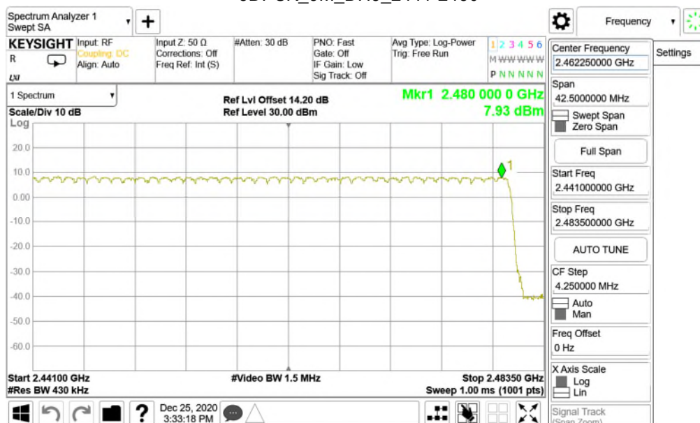
8DPSK_3M_DH5_2441-2480
