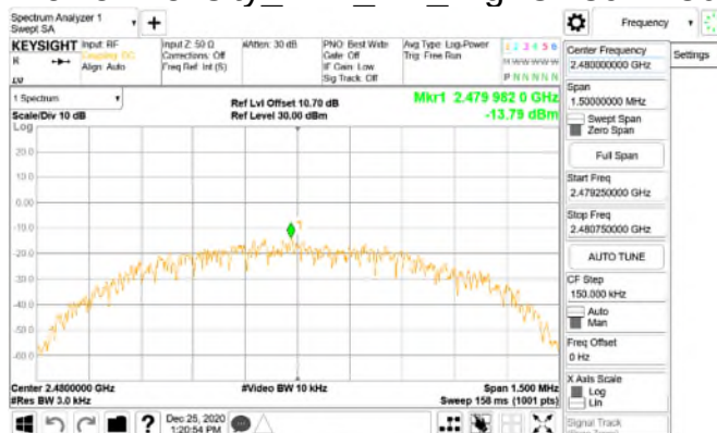
Power Density_BLE_1M_HighCH39-2480
