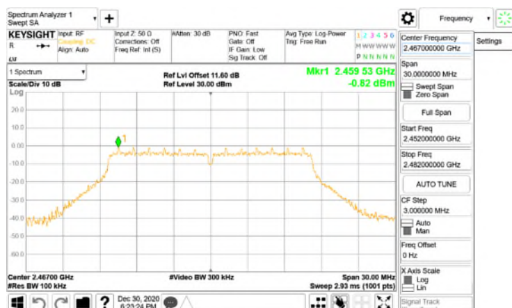
Reference Level\WLAN\802.11g_20MHz_Chain0_2467MHz
