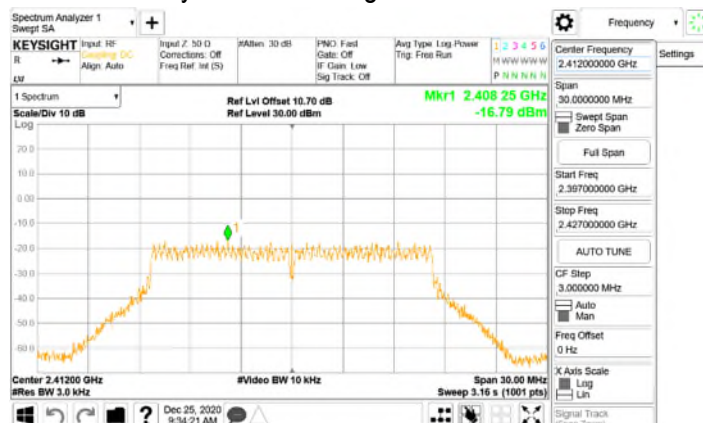
Power Density\WLAN\802.11g_20MHz_Chain0_2412MHz
