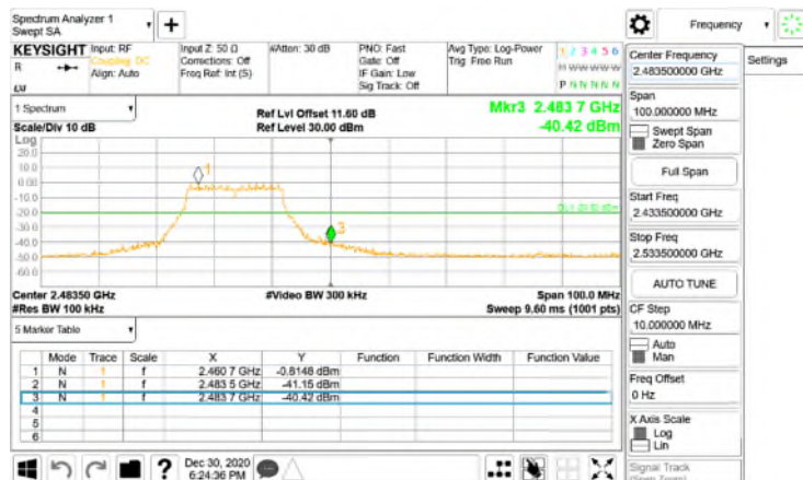
Band Edge\WLAN\802.11g_20MHz_Chain0_2472MHz
