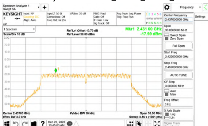
Power Density\WLAN\802.11n_20MHz_Chain0_2437MHz
