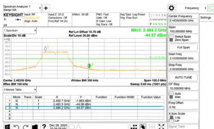
Band Edge\WLAN\802.11g_20MHz_Chain0_2462MHz
