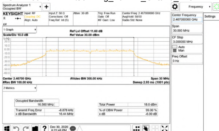
OBW 6dBWLAN\802.11g_20MHz_Chain0_2467MHz
