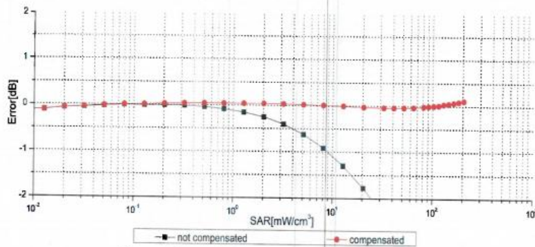
Uncertainty of Linearity Assessment: \pm 0.9\% ( k=2 )
