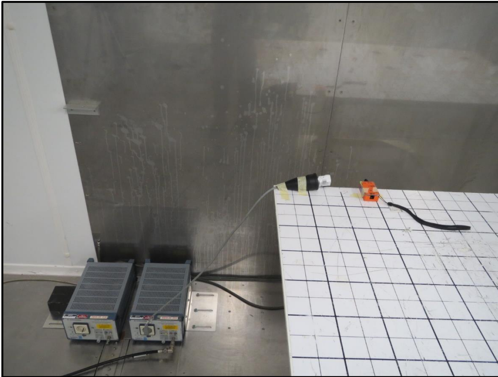
Photo 6 AC Conducted emission test setup
