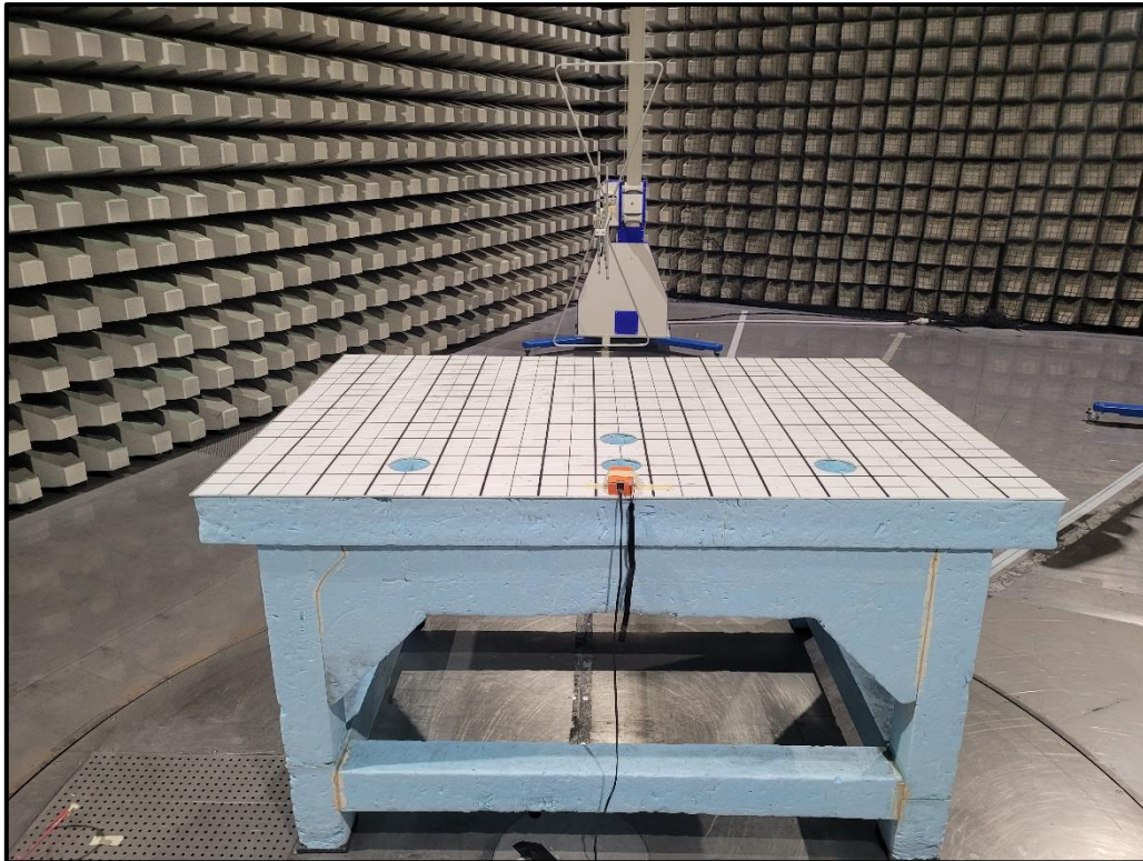
Photo 3 Radiated Test Setup from 30 MHz to 1 GHz
