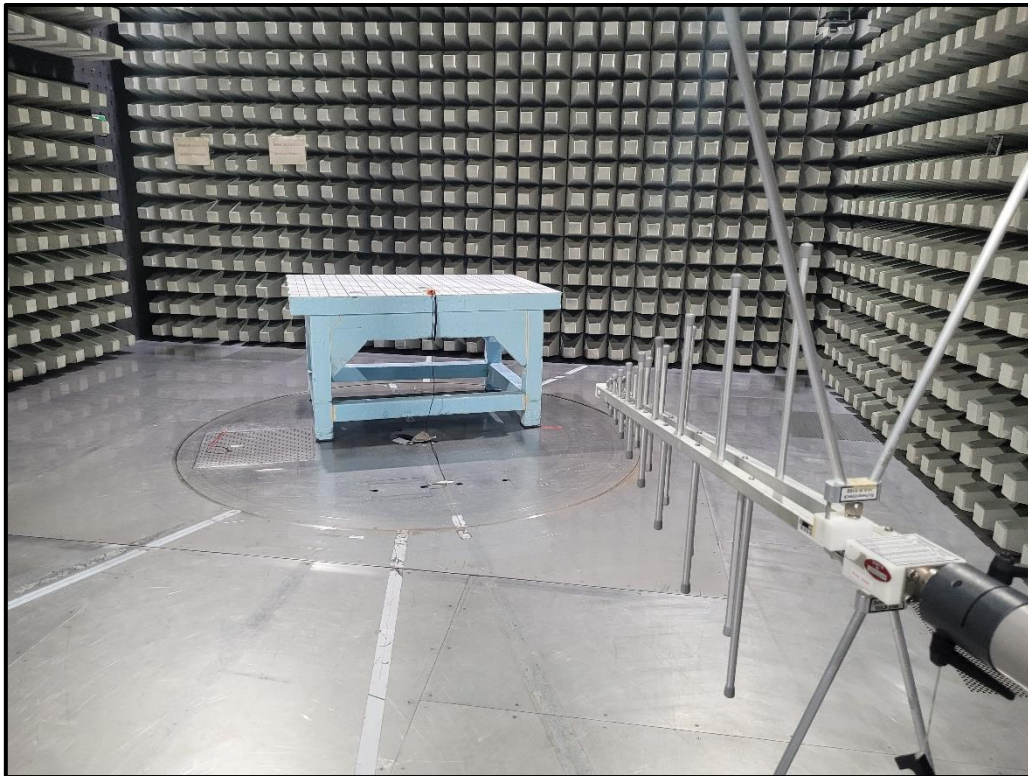
Photo 4 Radiated Test Setup from 30 MHz to 1 GHz
