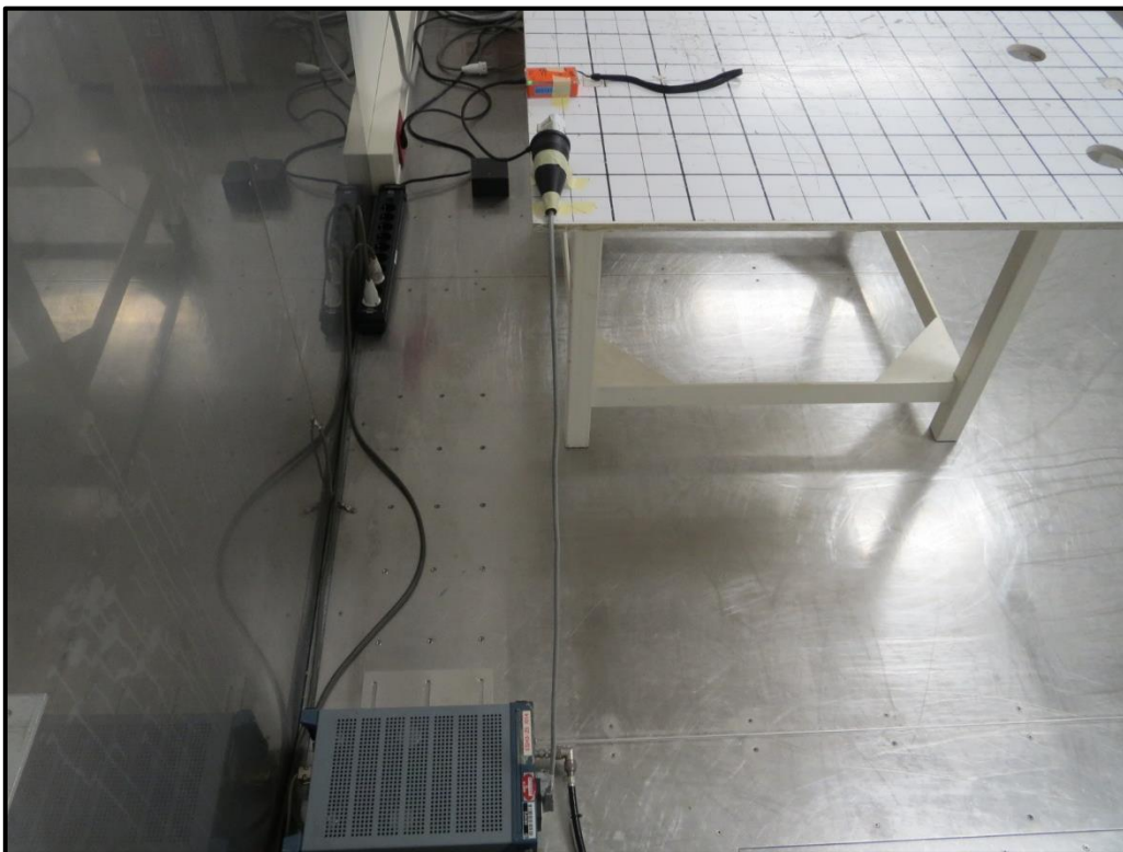
Photo 7 AC Conducted emission test setup
