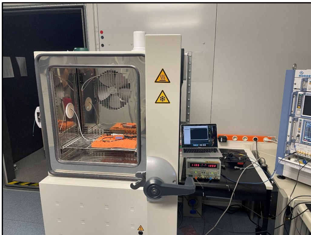
Photo 5 Coupling test setup
