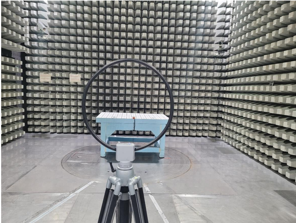
Photo 1 Radiated Test Setup below 30 MHz
