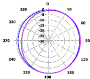
\phi = 0^\circ Plane XZ at 750 MHz, and 890MHz
