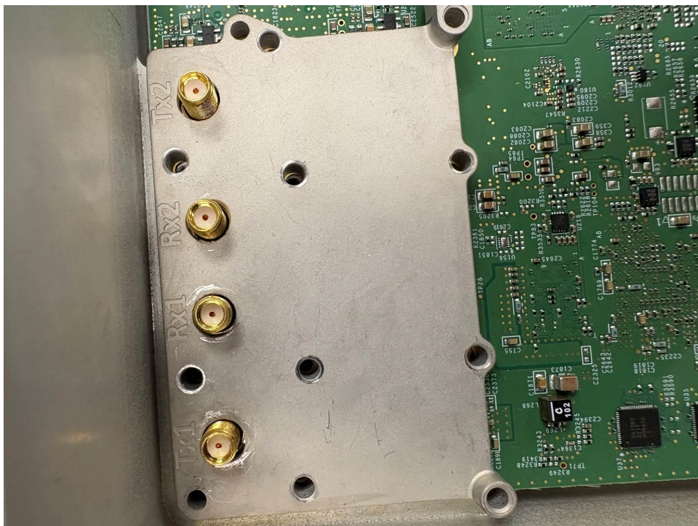
Close-up view LoRa radio shield
