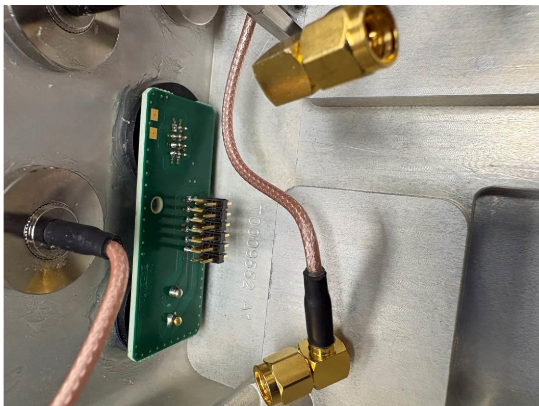
Close-up view of Ethernet / Power interface
