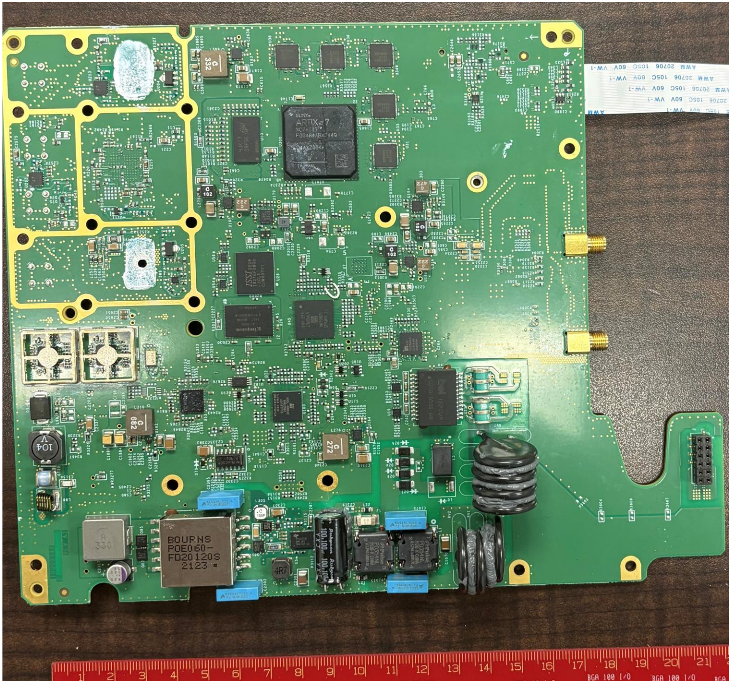
Main PCB bottom View:
