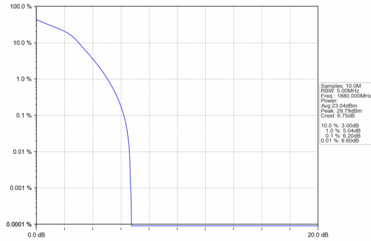
Band2 3MHz 16QAM MCH 1880MHz RB 15 0 NTN
