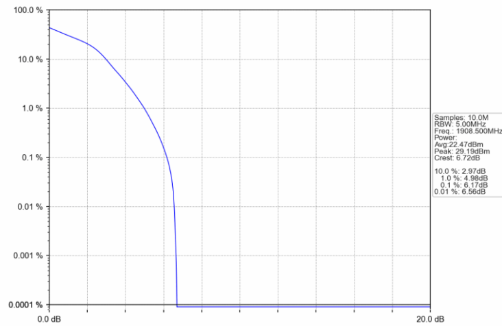
Band2 3MHz 16QAM HCH 1908.5MHz RB 15 0 NTN
