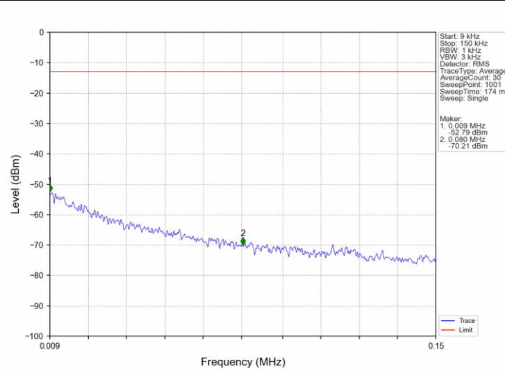
Band66_10MHz_16QAM_HCH_1775MHz_RB_1_0_NTNV
