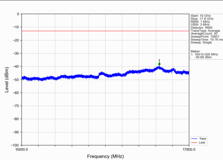
Band66_10MHz_16QAM_MCH_1745MHz_RB_1_0_NTNV
