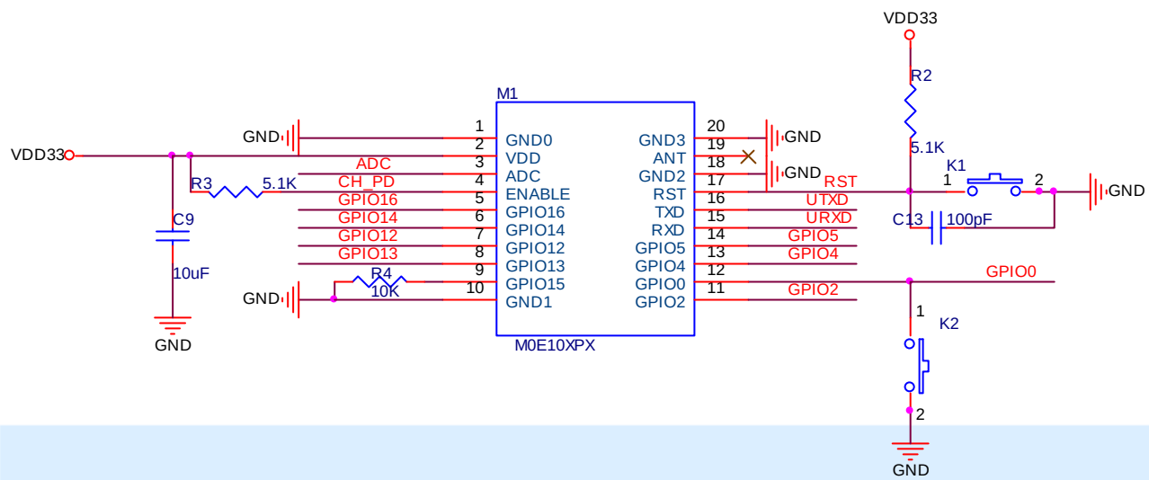
Figure 3. M0E10XPX Peripheral Schematics
