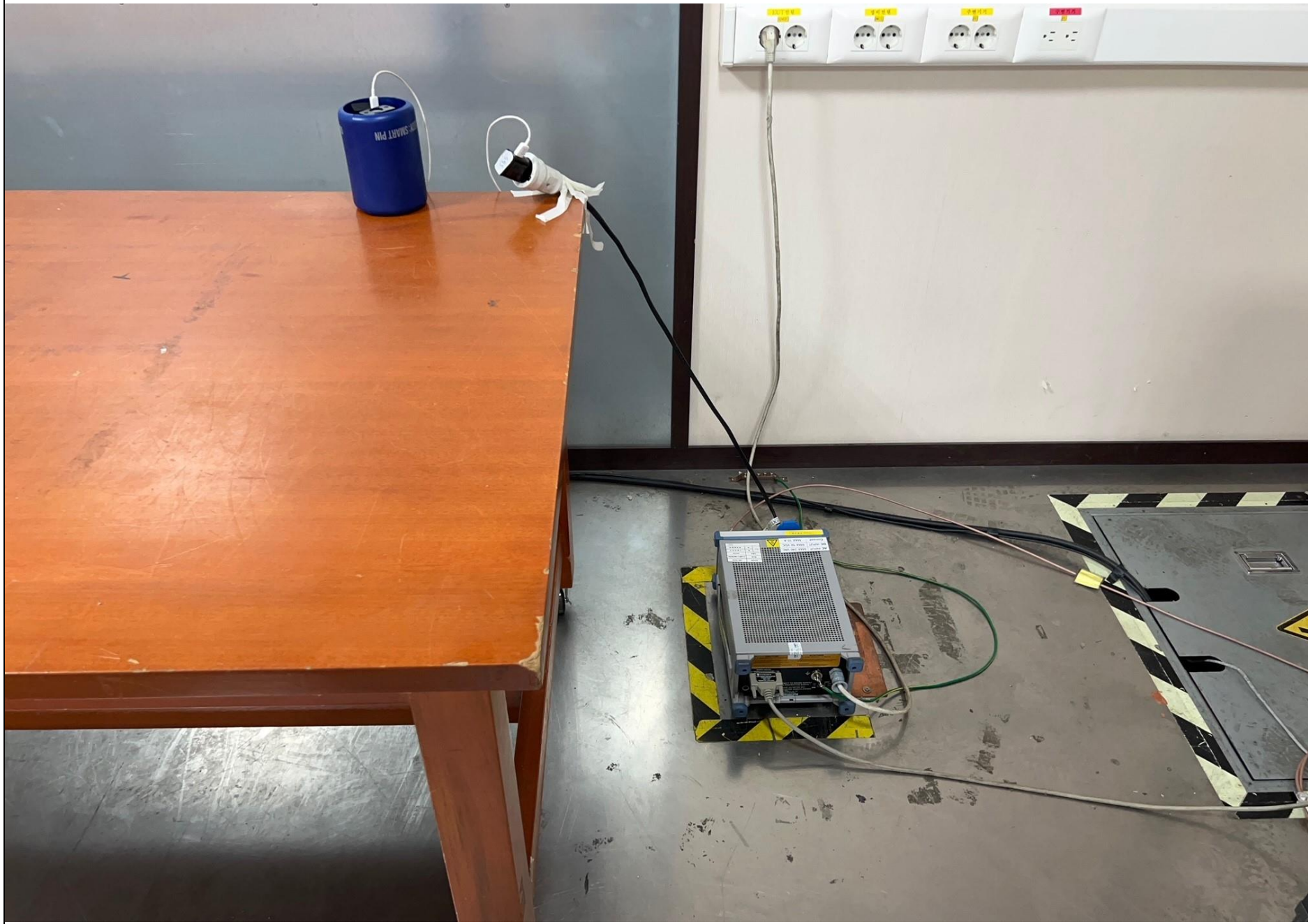
Continuous Conducted Emission at main _ Front
