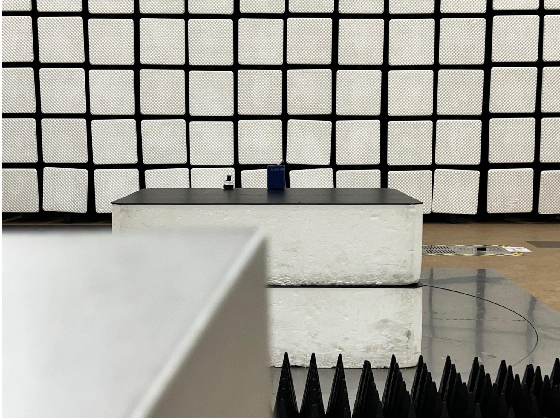
Radiated Emission (Above 1 GHz) _ Front
