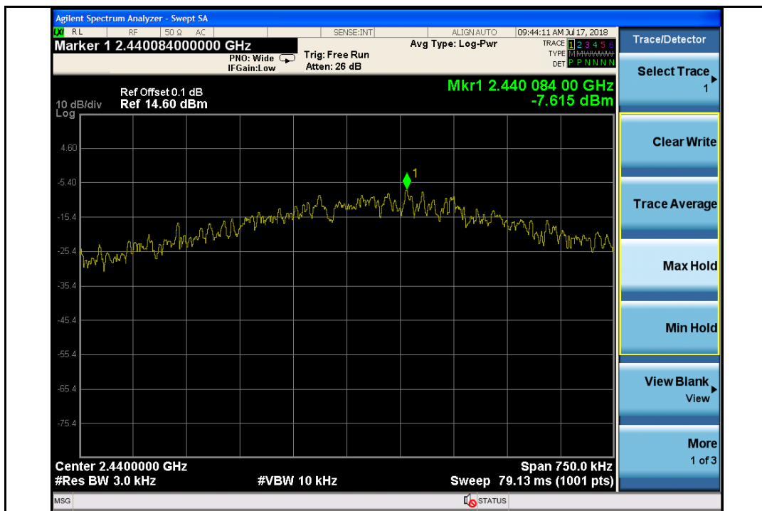
BLE-2440MHz-2Mbps
