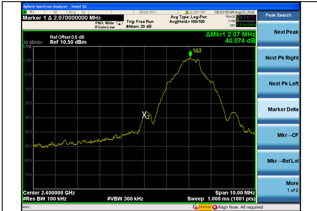
Conducted Band-Edge - BLE-2402MHz-2Mbps
