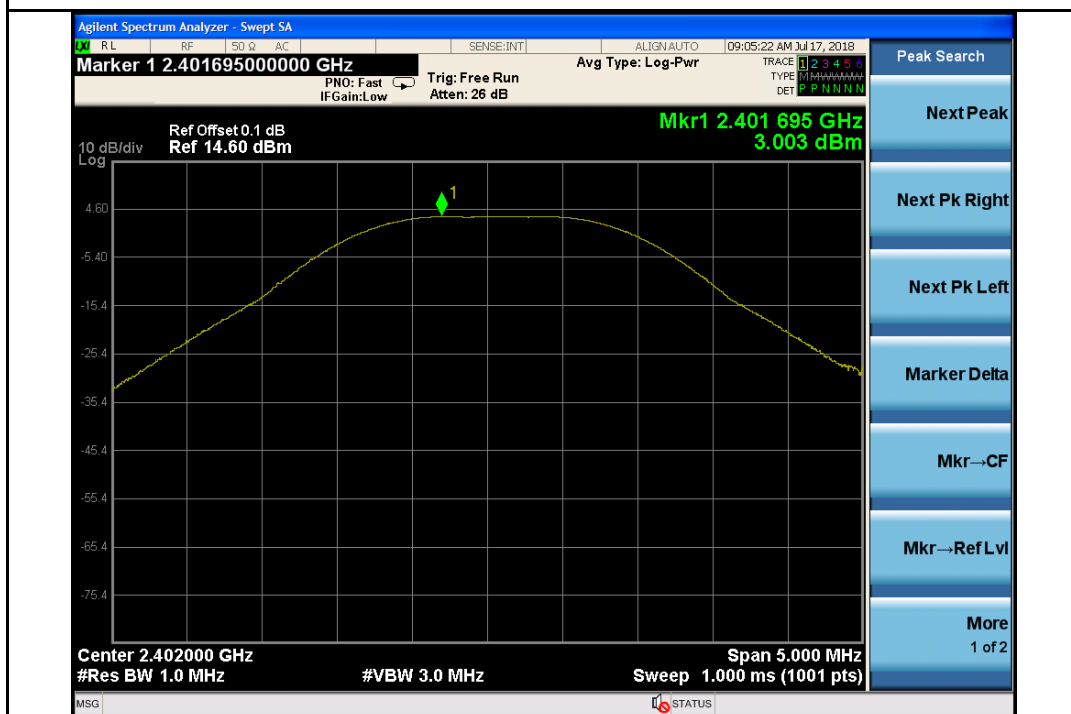
BLE-2402MHz-2Mbps
