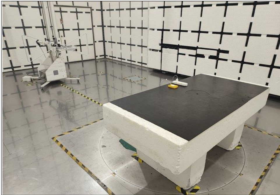
RADIATED EMISSION TEST BELOW 1GHz
