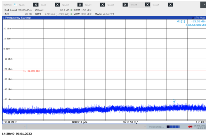
Figure 8.6-7: Conducted spurious emissions 30-1000 MHz on High ch.
