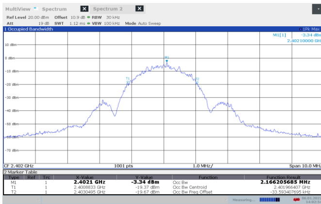
Figure 8.4-4: 99% occupied bandwidth on Low ch.
