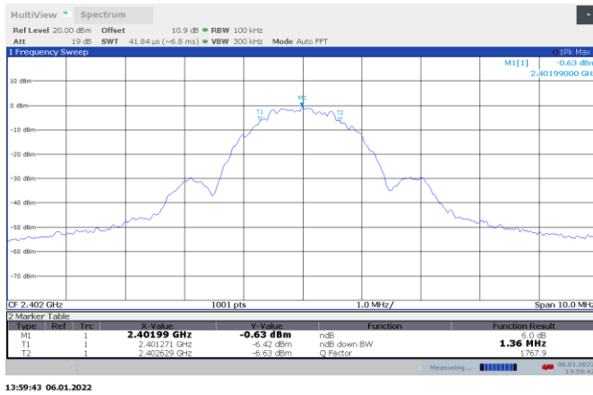
Figure 8.4-1: 6 dB bandwidth on Low ch.
