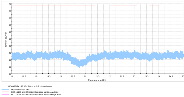
Figure 8.6-19: Radiated spurious emissions 18- 25 GHz on Low ch
