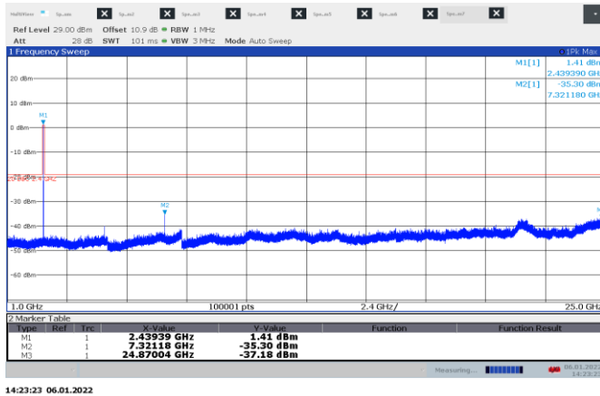
Figure 8.6-9: Conducted spurious emissions 1-25 GHz on Mid ch.
