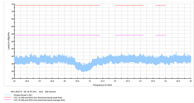
Figure 8.6-20: Radiated spurious emissions 18- 25 GHz on Mid ch
