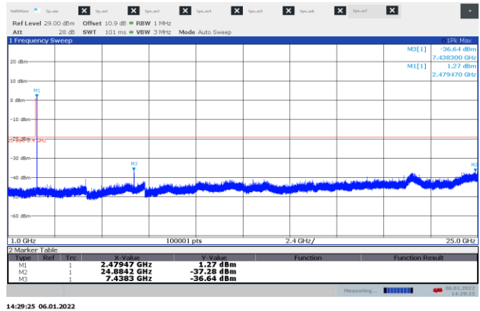
Figure 8.6-10: Conducted spurious emissions 1-25 GHz on High ch.
