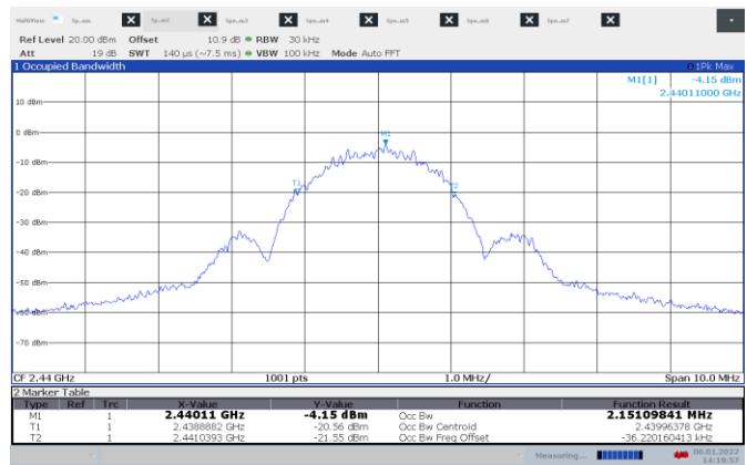
Figure 8.4-5: 99% occupied bandwidth on Mid ch.
