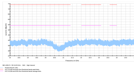
Figure 8.6-21: Radiated spurious emissions 18- 25 GHz on High ch
