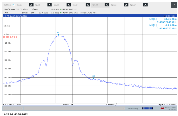
Figure 8.6-12: Conducted band edge outside of-restricted band On High ch.
