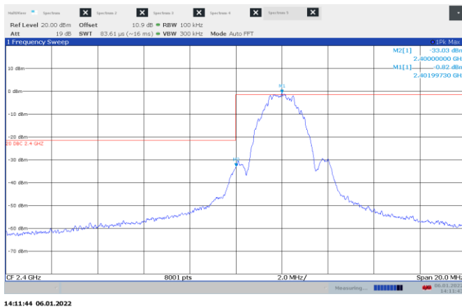
Figure 8.6-11: Conducted band edge outside of-restricted band On Low ch.
