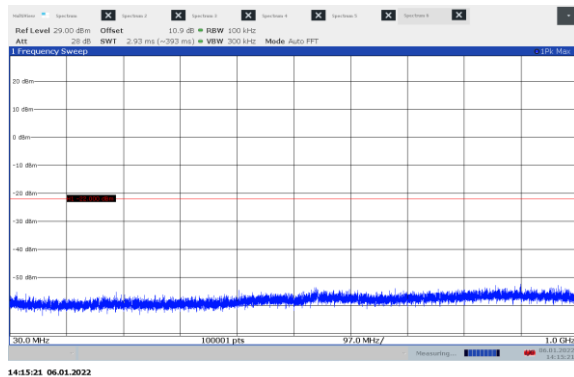
Figure 8.6-5: Conducted spurious emissions 30-1000 MHz on Low ch.
