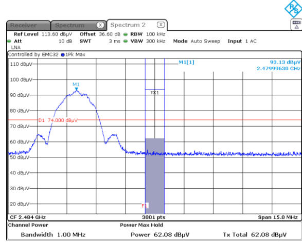
Figure 8.6-2: Band edge spurious emissions at 2483.5 MHz Peak
