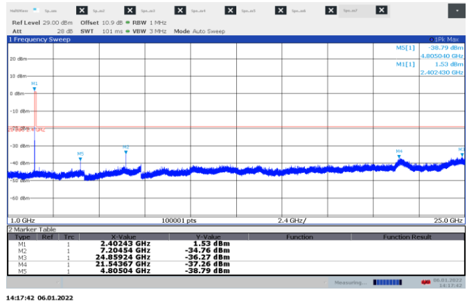
Figure 8.6-8: Conducted spurious emissions 1-25 GHz on Low ch.
