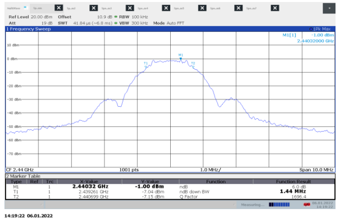
Figure 8.4-2: 6 dB bandwidth on Mid ch.
