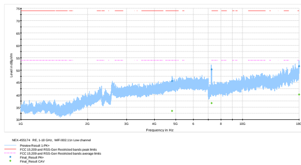
Figure 8.6-37: Radiated spurious emissions 1- 18 GHz on Low ch.
