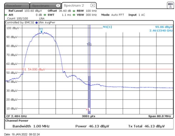
Figure 8.6-4: Band edge spurious emissions at 2483.5 MHz Average
