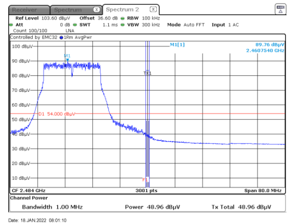
Figure 8.6-18: Band edge spurious emissions at 2483.5 MHz Average
