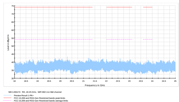
Figure 8.6-40: Radiated spurious emissions 18- 25 GHz on Mid ch, sample plot
