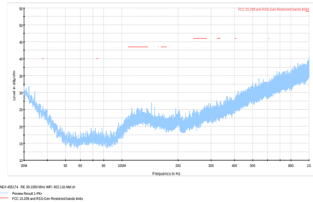
Figure 8.6-8: Radiated spurious emissions 30- 1000 MHz on Mid ch, sample plot
