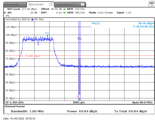
Figure 8.6-16: Band edge spurious emissions at 2483.5 MHz Peak
