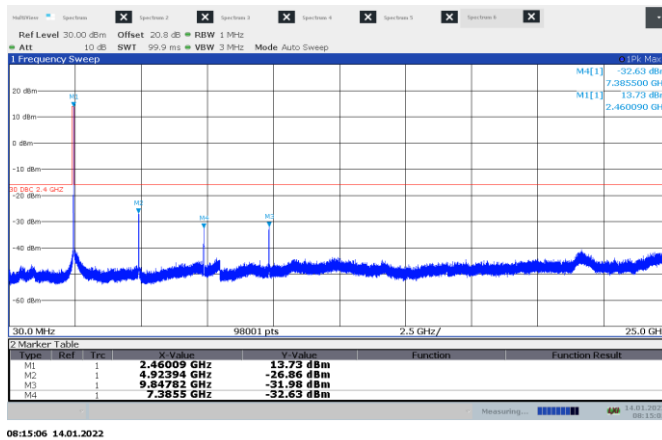
Figure 8.6-7: Conducted spurious emissions 30 MHz-25 GHz on High ch.
