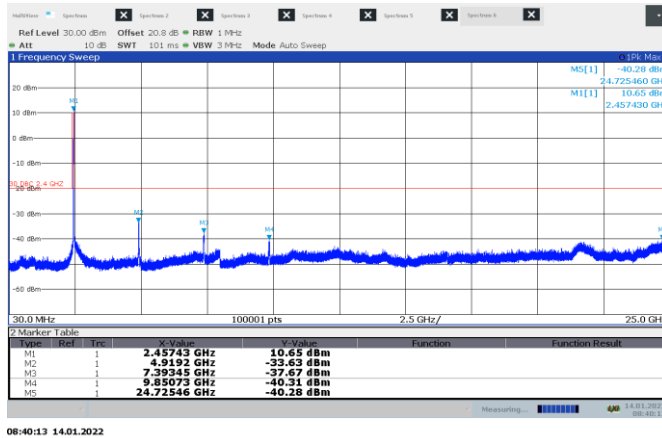
Figure 8.6-21: Conducted spurious emissions 30 MHz-25 GHz on High ch.
