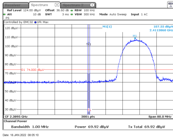
Figure 8.6-1: Band edge spurious emissions at 2390 MHz Peak
