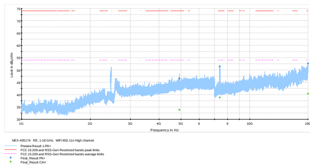
Figure 8.6-39: Radiated spurious emissions 1- 18 GHz on High ch
