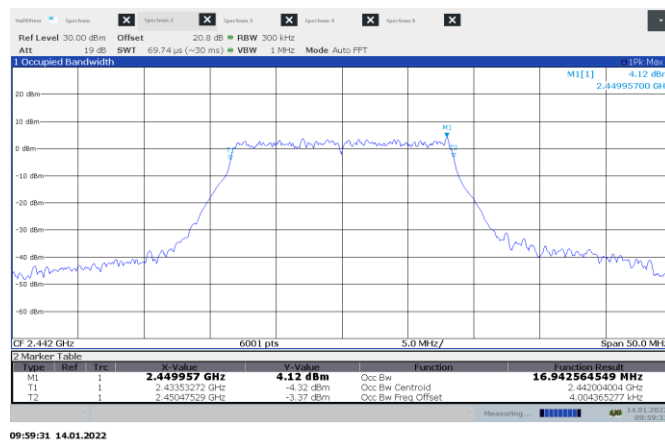
Figure 8.4-5: 99% occupied bandwidth on 802.11g, sample plot
