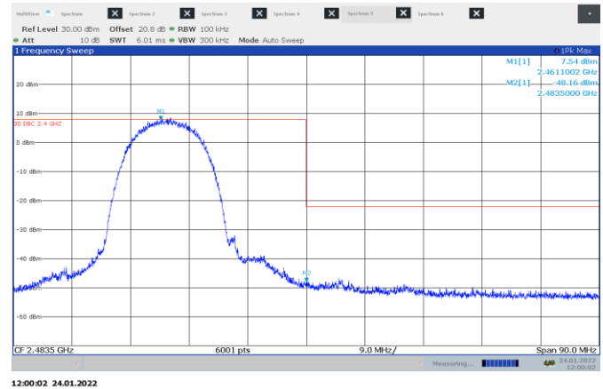
Figure 8.6-14: Conducted emissions in non-restricted band on High ch
