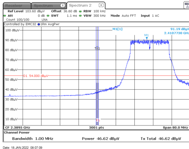
Figure 8.6-17: Band edge spurious emissions at 2390 MHz Average
