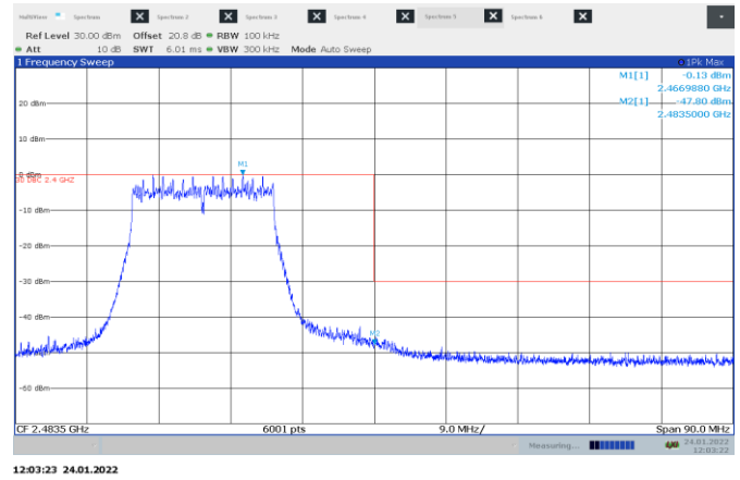
Figure 8.6-42: Conducted emissions in non-restricted band on High ch
