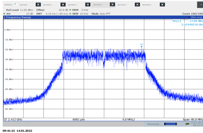
Figure 8.7-4: PSD on low channel, 802.11g
