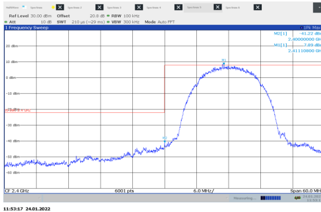
Figure 8.6-13: Conducted emissions in non-restricted band on Low ch.
