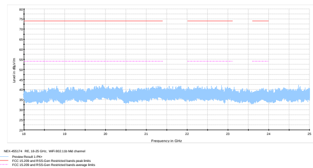
Figure 8.6-12: Radiated spurious emissions 18- 25 GHz on Mid ch, sample plot
