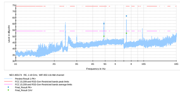
Figure 8.6-10: Radiated spurious emissions 1- 18 GHz on Mid ch
