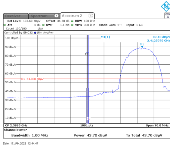
Figure 8.6-3: Band edge spurious emissions at 2390 MHz Average
