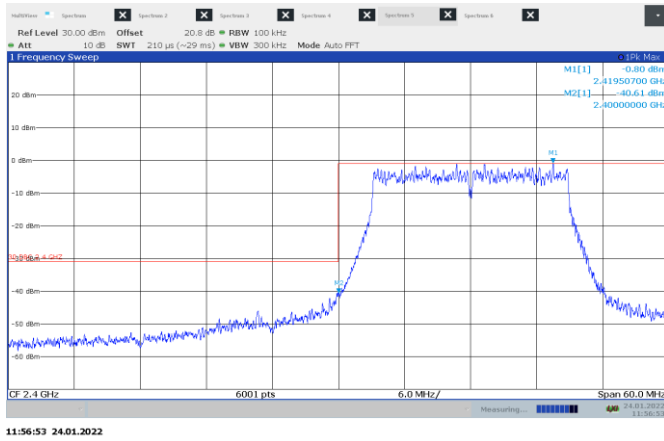
Figure 8.6-41: Conducted emissions in non-restricted band on Low ch.
