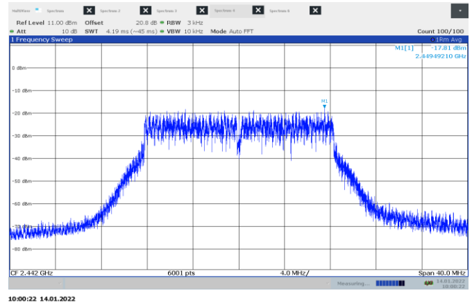
Figure 8.7-5: PSD on mid channel, 802.11g
