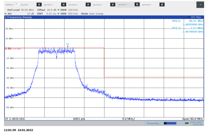
Figure 8.6-28: Conducted emissions in non-restricted band on High ch
