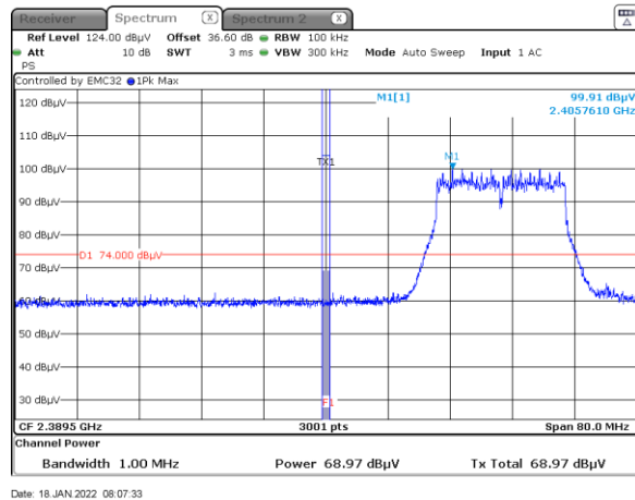
Figure 8.6-15: Band edge spurious emissions at 2390 MHz Peak
