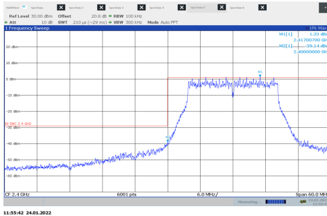
Figure 8.6-27: Conducted emissions in non-restricted band on Low ch.
