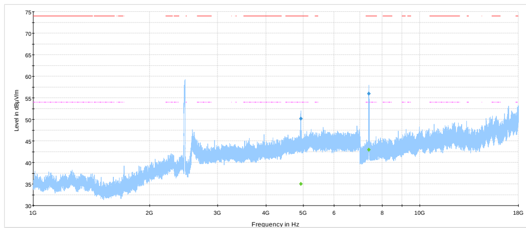
Figure 8.1-3: Radiated spurious emissions 1- 18 GHz on Mid ch
