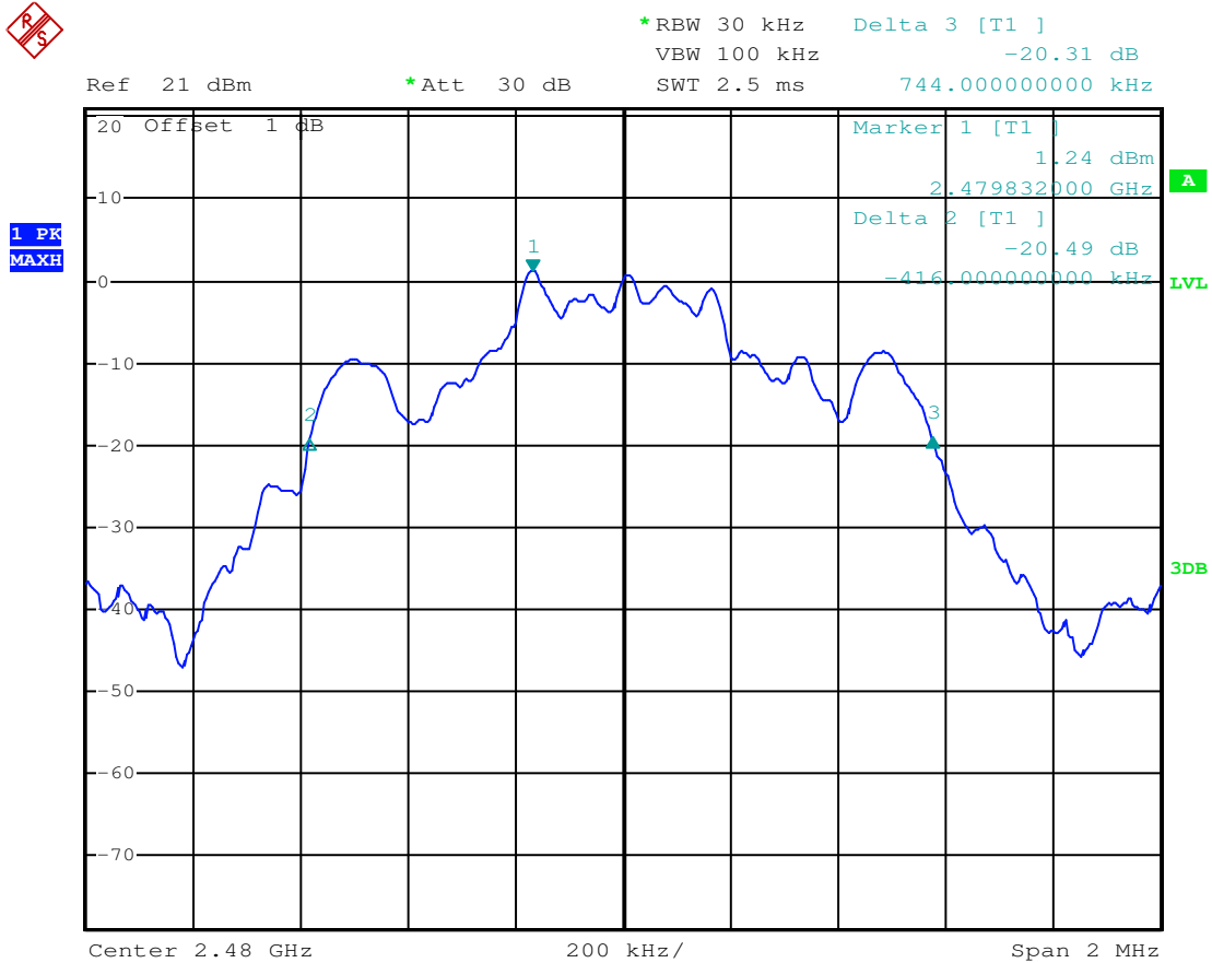
(Plot 4.4.2 C: Channel 78: 2480MHz @ 8DPSK)
