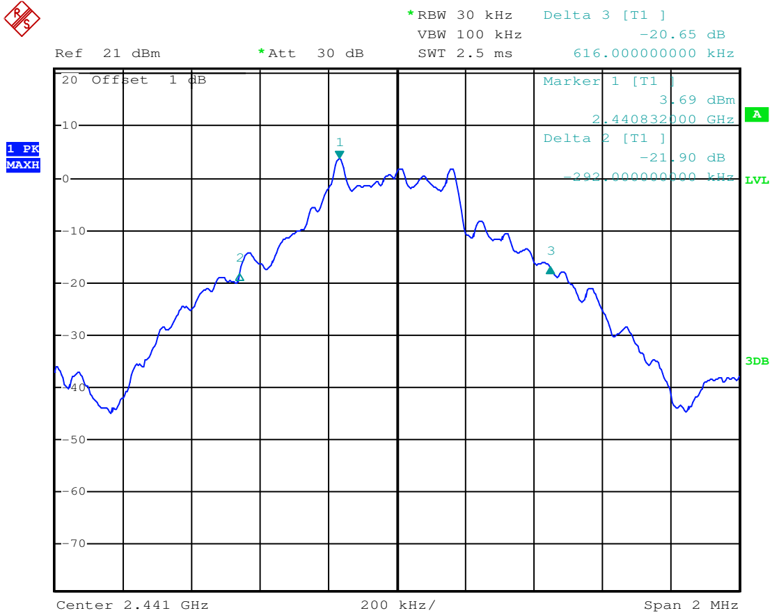
(Plot 4.4.1 B: Channel 39: 2441MHz @ GFSK)
