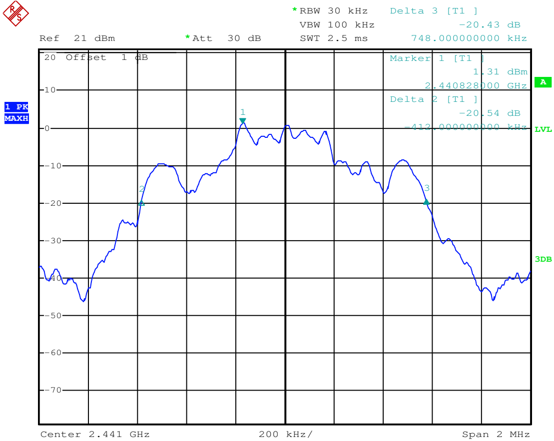
(Plot 4.4.2 B: Channel 39: 2441MHz @ 8DPSK)
