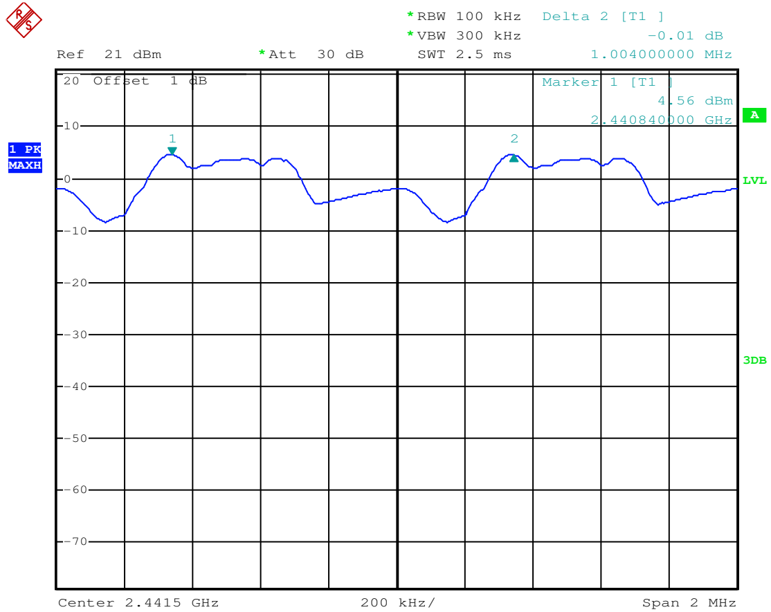
(Plot 4.5.2 A: Channel 39: 2441MHz @ 8DPSK)
