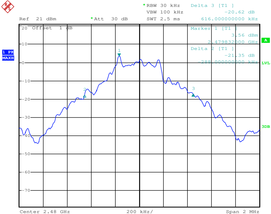
(Plot 4.4.1 C: Channel 78: 2480MHz @ GFSK)
