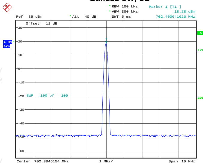
Band12 CW, UL
