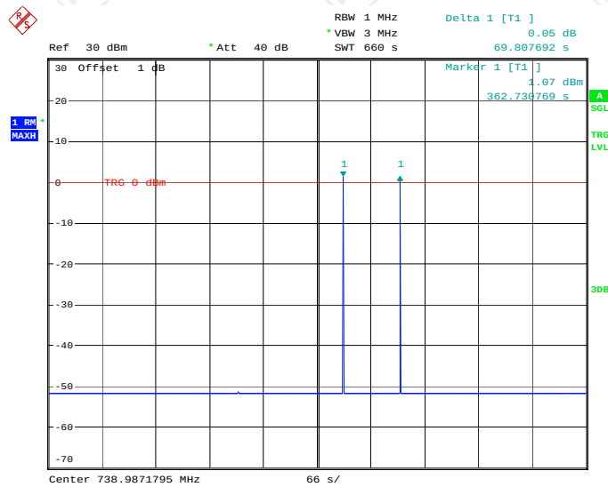
Band12 DL
