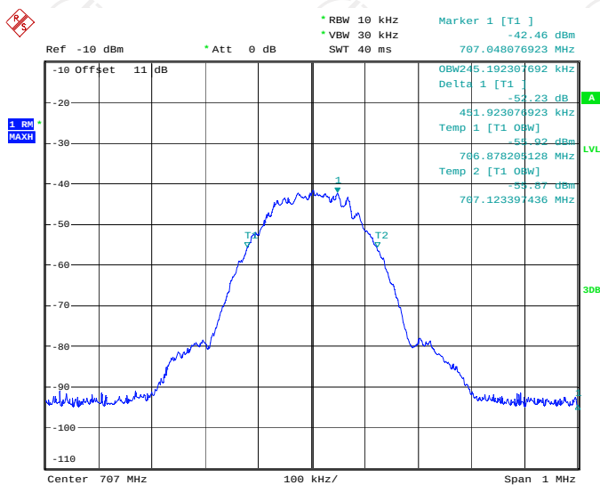
Band12 GSM UL Input
