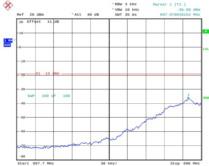
Band12 GSM UL Left Side Pre AGC
