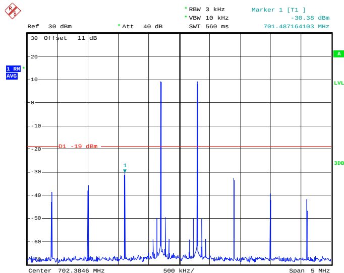
Band12 Pre AGC, UL
