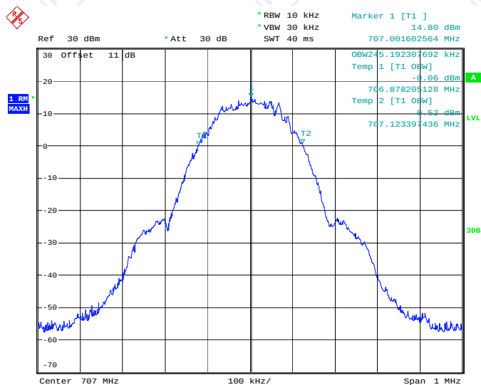
Band12 GSM UL output
