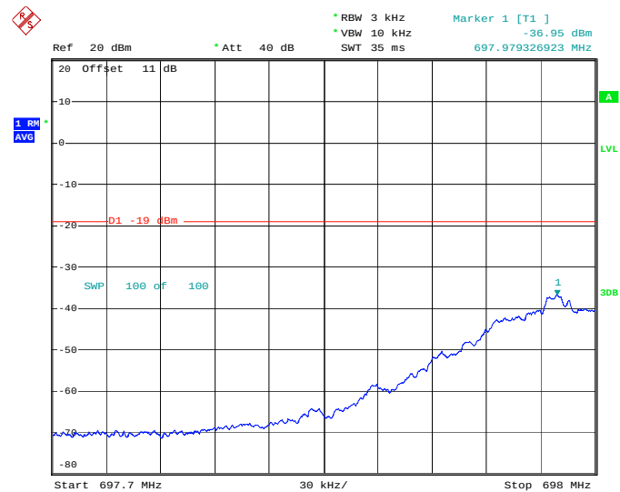
Band12 GSM UL Left Side Max. Input
