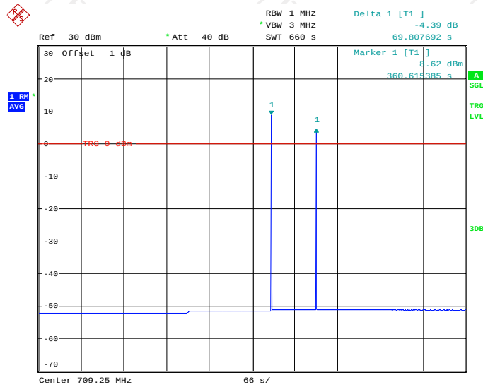
Band12 UL
