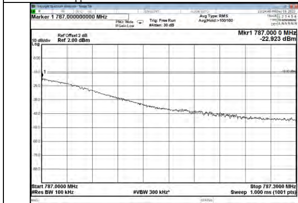
Upper 700MHz band LTE UL Right Side Pre AGC
