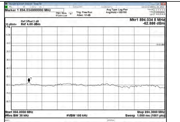
Cellular Band CDMA DL Right Side 10dB Above AGC
