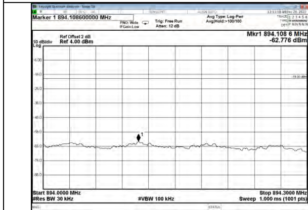
Cellular Band CDMA DL Right Side Pre AGC
