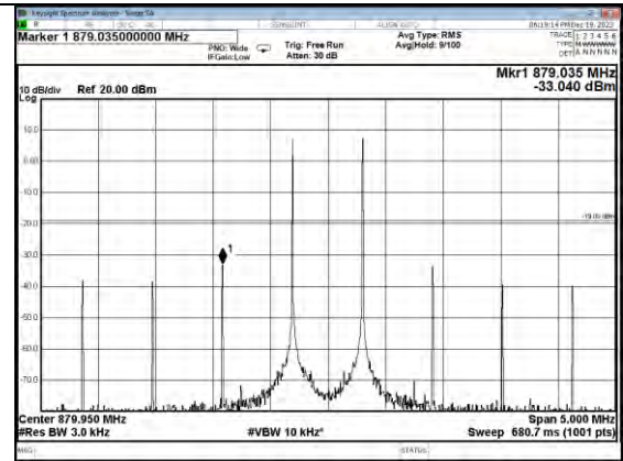
Cellular Band AGC+10dB, DL
