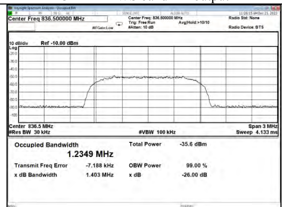
CDMA-Cellular band UL output
