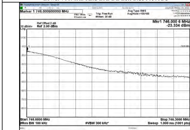
Lower 700MHz band LTE DL Right Side Pre AGC
