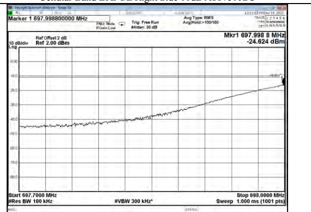
Lower 700MHz band LTE UL Left Side 10dB Above AGC
