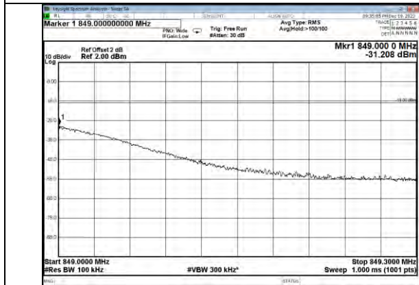
Cellular Band LTE UL Right Side Pre AGC
