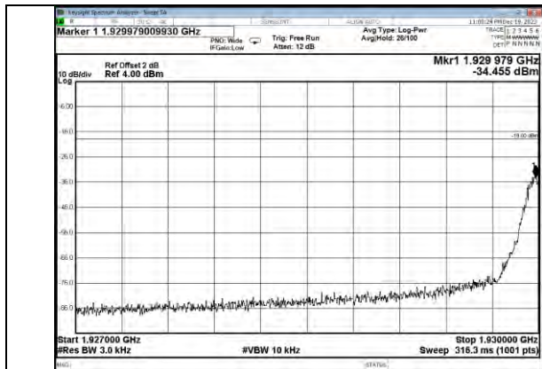
PCS Band GSM DL Left Side Pre AGC
