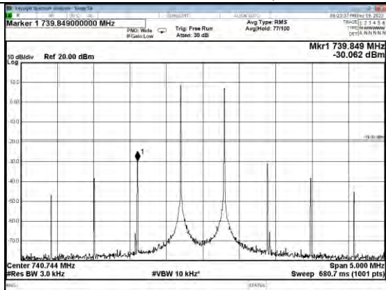
Lower 700MHz band Pre AGC, DL
