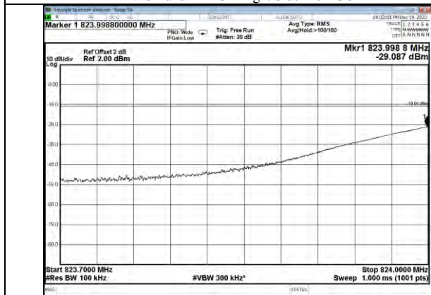
Cellular Band LTE UL Left Side Pre AGC
