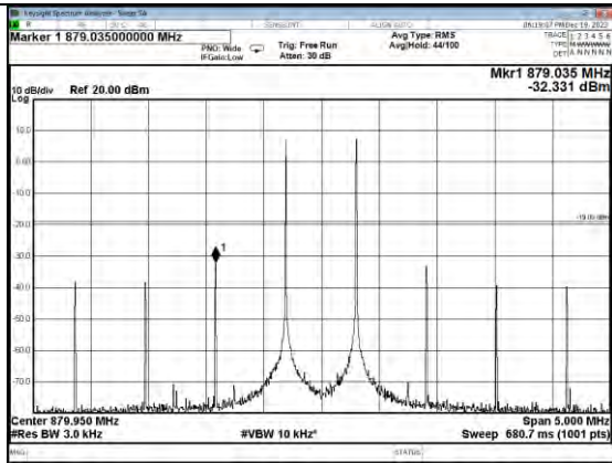
Cellular Band Pre AGC, DL
