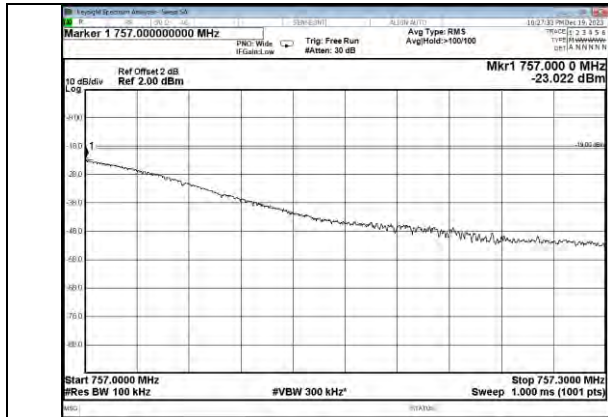
Upper 700MHz band LTE DL Right Side Pre AGC
