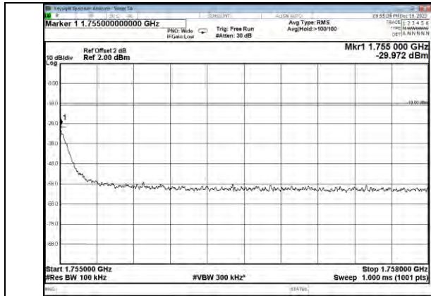
AWS Band LTE UL Right Side Pre AGC
