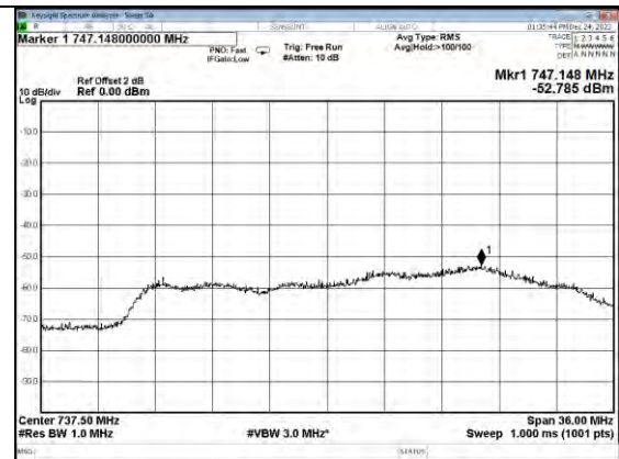
Lower 700MHz band DL
