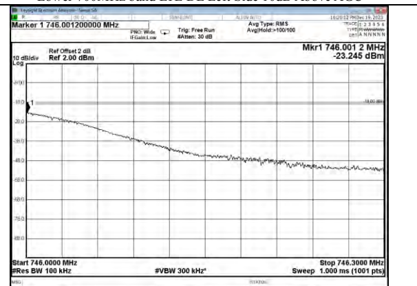
Lower 700MHz band LTE DL Right Side 10dB Above AGC
