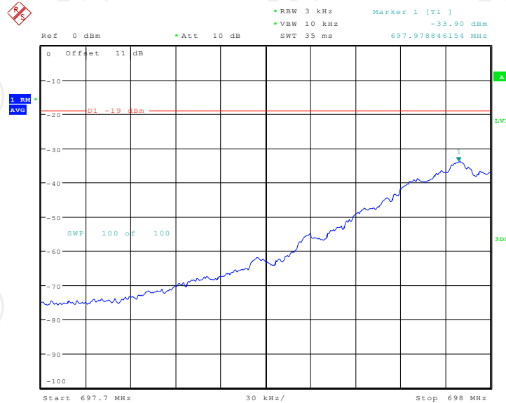
Lower700MHz GSM UL Left Side Pre AGC
