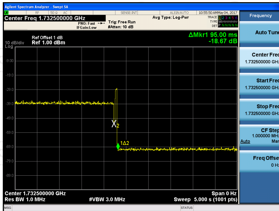
Uplink_1732.5MHz
