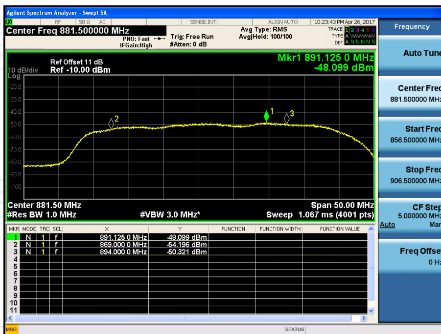
Downlink Noise:869~894MHz
