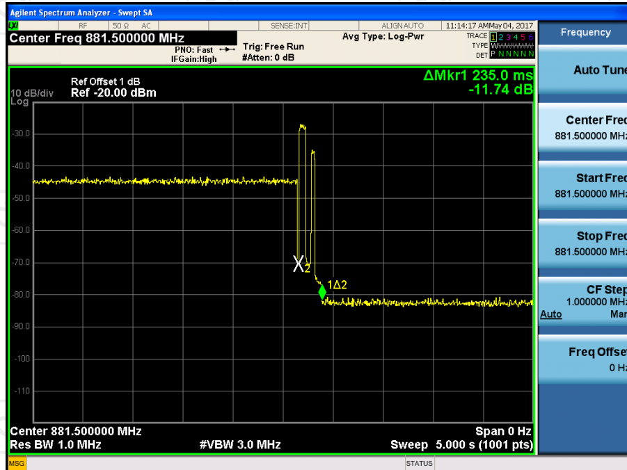
Downlink_881.5MHz
