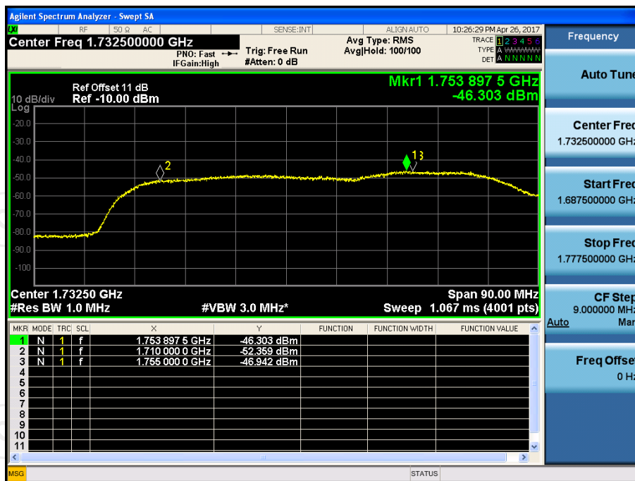
Uplink Noise:1710~1755MHz
