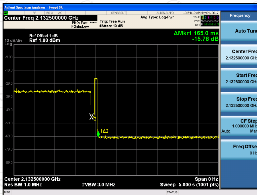
Downlink_2132.5MHz
