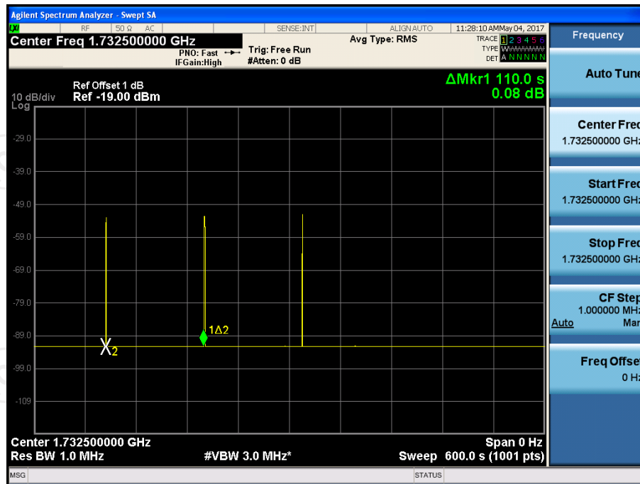
Uplink_1732.5MHz
