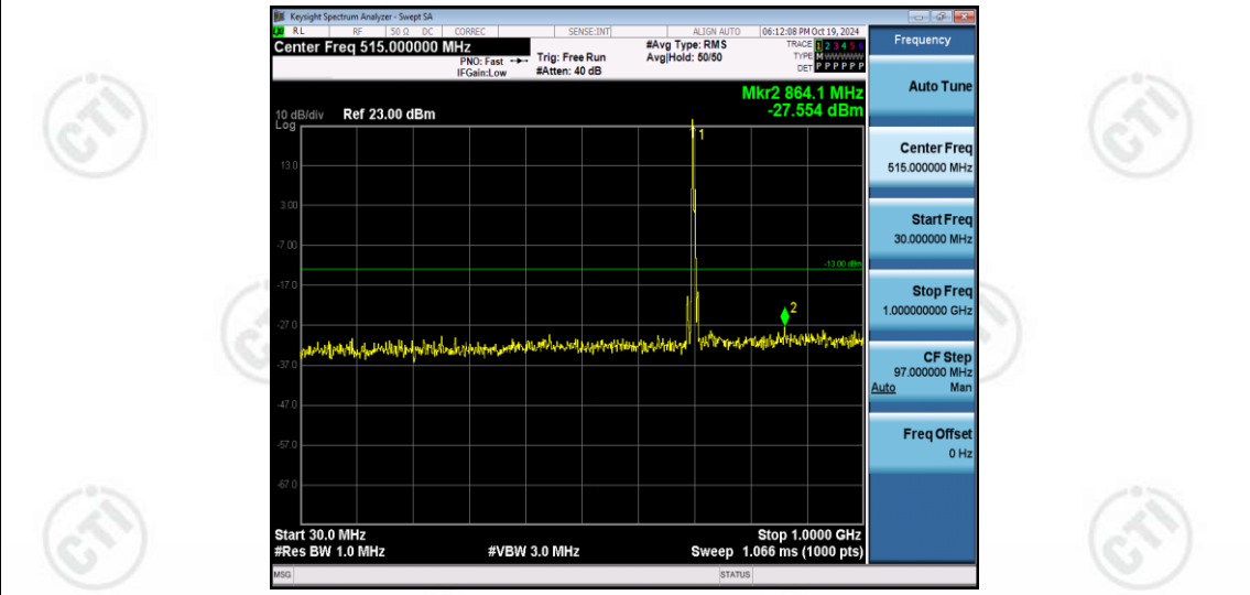
Band12-5MHz-16QAM-23095-1RB#0-Range1:30~1000MHz
