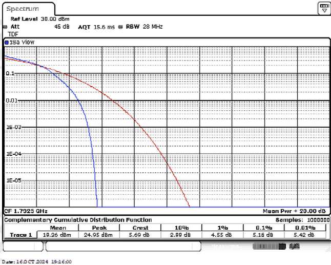
Band4-3MHz-16QAM-20175-15RB#0
