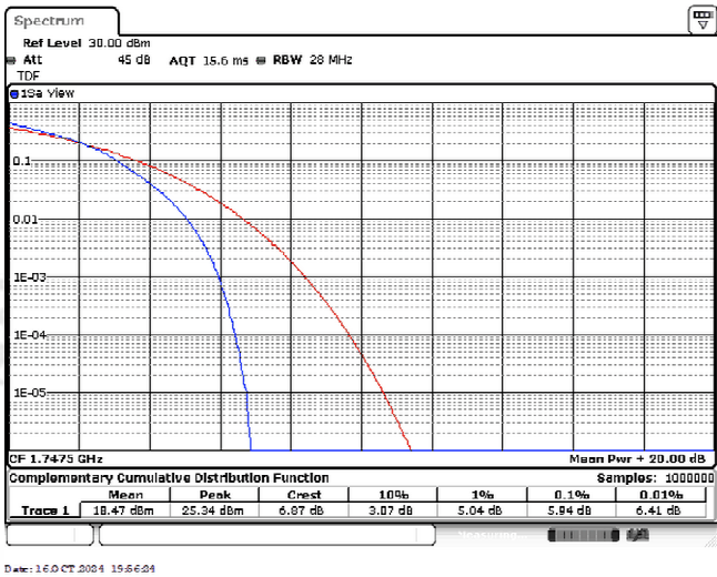
Band4-15MHz-16QAM-20325-25RB#0
