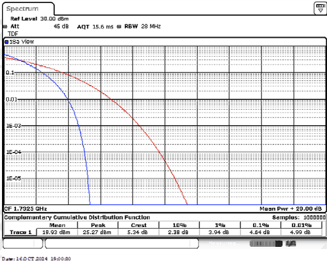
Band4-20MHz-QPSK-20175-100RB#0
