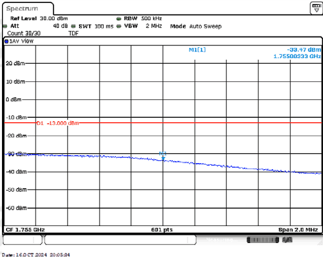
Band4-20MHz-16QAM-20300-1RB#24
