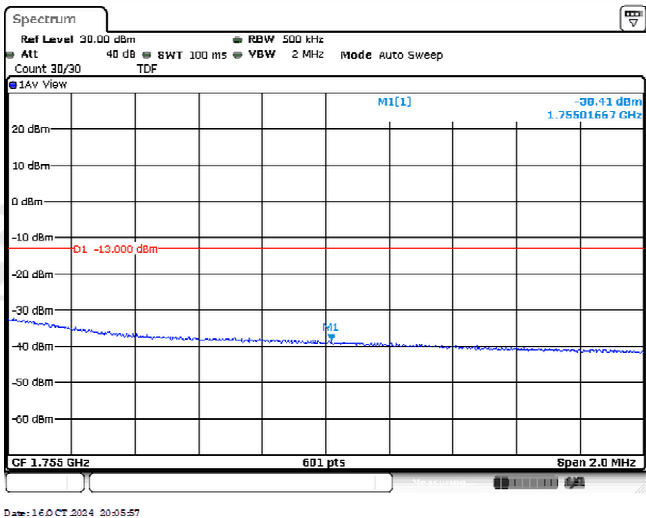
Band4-20MHz-16QAM-20300-25RB#0
